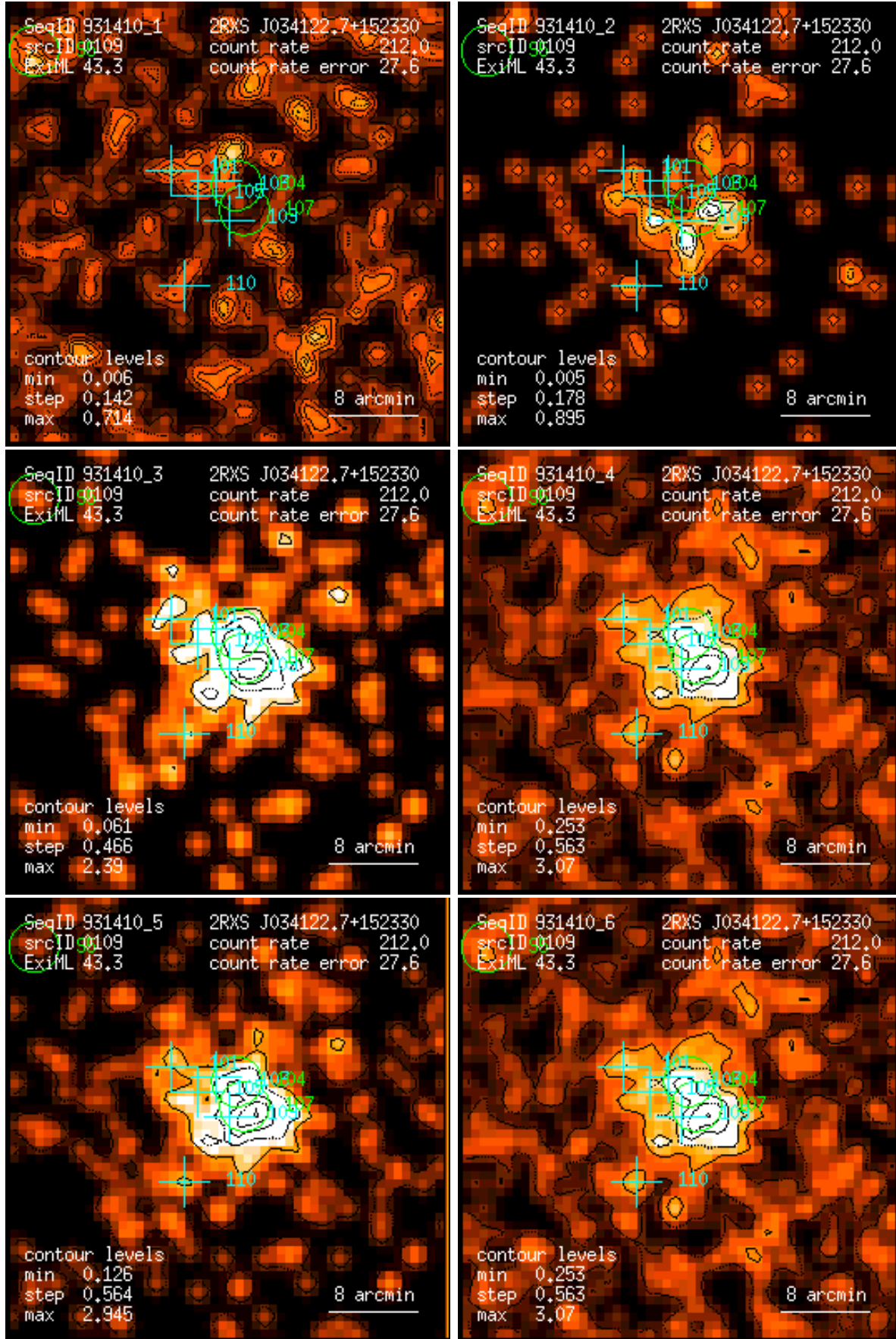
Figure 109: RASS 931410: detection 0109: band rate images, Gaussian filter: (1) PSPC channels 11 – 41, (2) 52 – 90, (3) 91 – 201, (4) 11 – 235, (5) 52 – 201, (6) 11 – 201. Broad band rates in counts/ks. Band rate contour levels in counts/ks/arcmin 2 .
