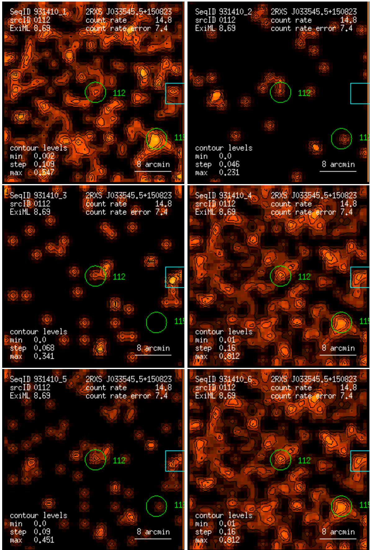
Figure 112: RASS 931410: detection 0112: band rate images, Gaussian filter: (1) PSPC channels 11 – 41, (2) 52 – 90, (3) 91 – 201, (4) 11 – 235, (5) 52 – 201, (6) 11 – 201. Broad band rates in counts/ks. Band rate contour levels in counts/ks/arcmin 2 .
