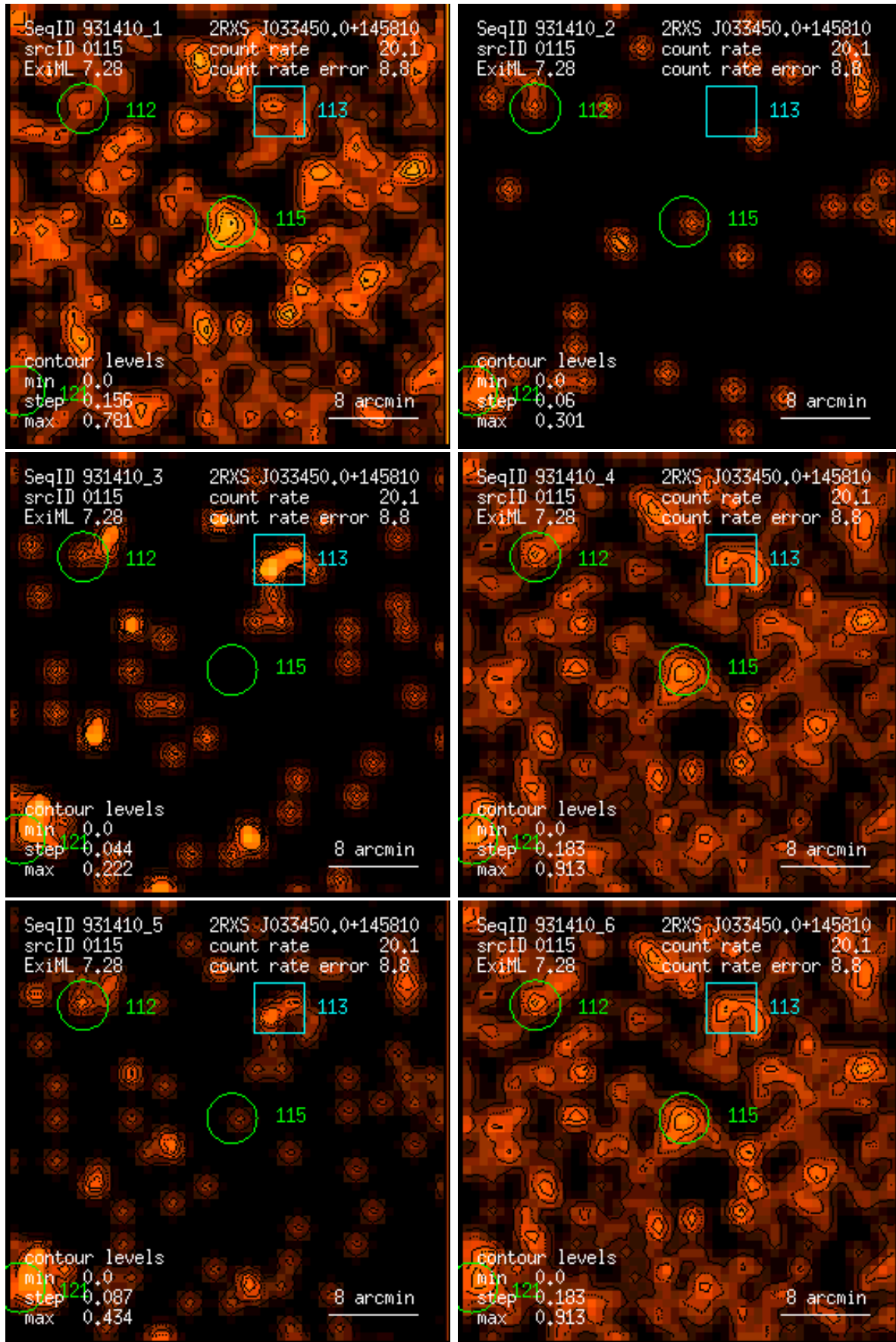
Figure 115: RASS 931410: detection 0115: band rate images, Gaussian filter: (1) PSPC channels 11 – 41, (2) 52 – 90, (3) 91 – 201, (4) 11 – 235, (5) 52 – 201, (6) 11 – 201. Broad band rates in counts/ks. Band rate contour levels in counts/ks/arcmin 2 .
