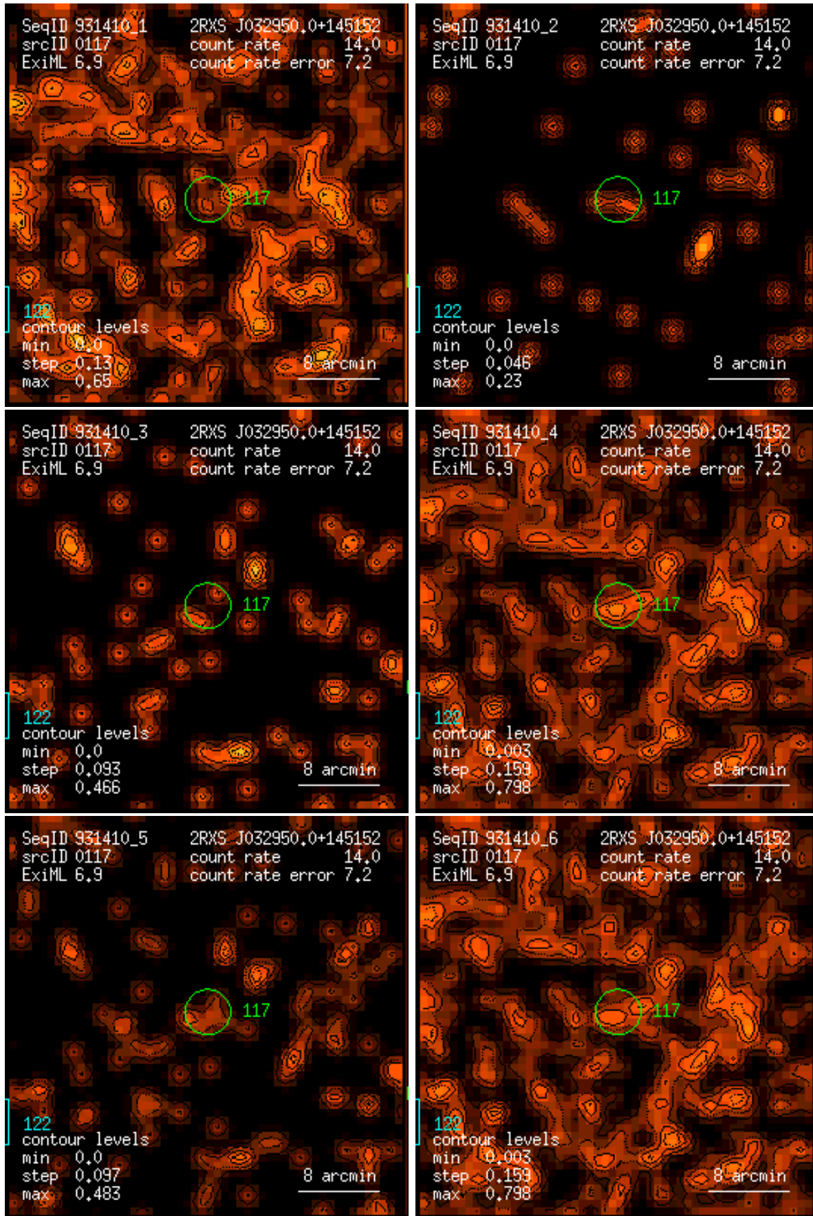
Figure 117: RASS 931410: detection 0117: band rate images, Gaussian filter: (1) PSPC channels 11 – 41, (2) 52 – 90, (3) 91 – 201, (4) 11 – 235, (5) 52 – 201, (6) 11 – 201. Broad band rates in counts/ks. Band rate contour levels in counts/ks/arcmin 2 .
