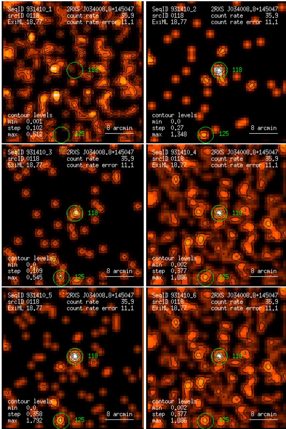
Figure 118: RASS 931410: detection 0118: band rate images, Gaussian filter: (1) PSPC channels 11 – 41, (2) 52 – 90, (3) 91 – 201, (4) 11 – 235, (5) 52 – 201, (6) 11 – 201. Broad band rates in counts/ks. Band rate contour levels in counts/ks/arcmin 2 .
