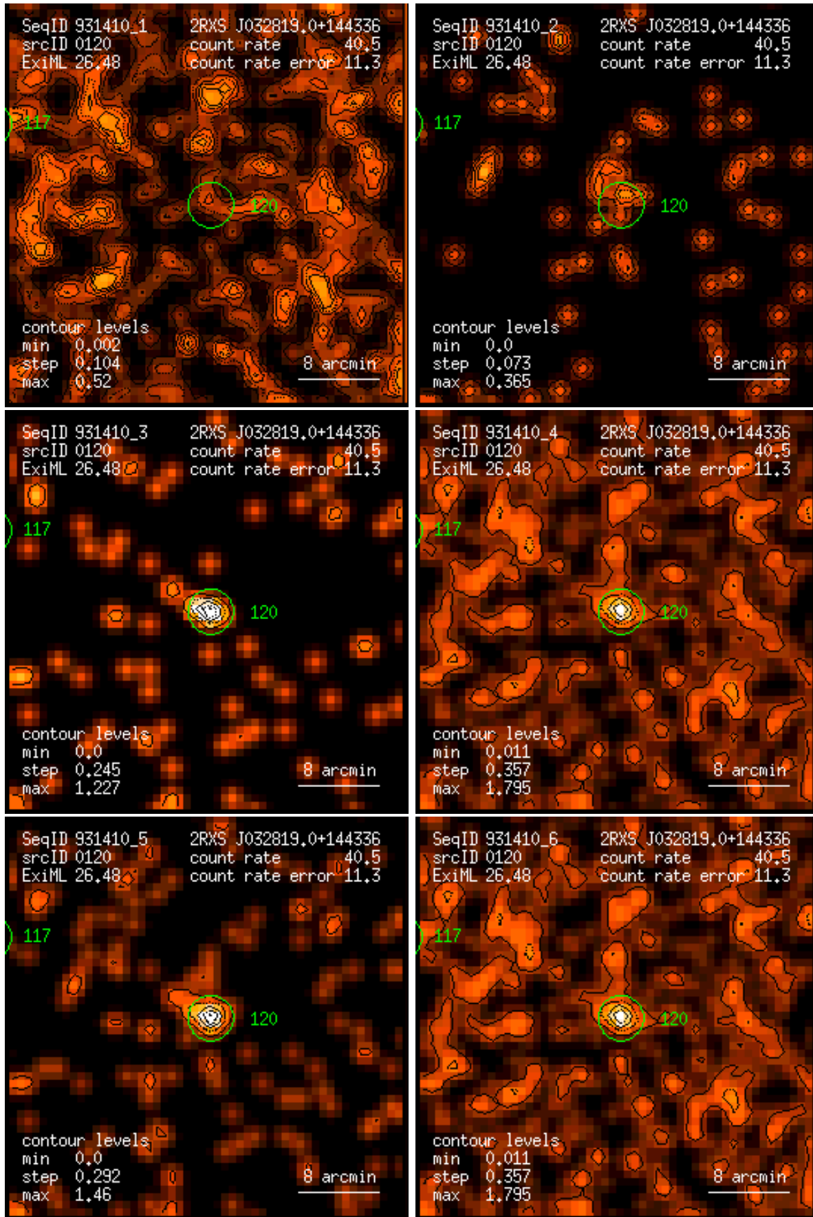
Figure 120: RASS 931410: detection 0120: band rate images, Gaussian filter: (1) PSPC channels 11 – 41, (2) 52 – 90, (3) 91 – 201, (4) 11 – 235, (5) 52 – 201, (6) 11 – 201. Broad band rates in counts/ks. Band rate contour levels in counts/ks/arcmin 2 .
