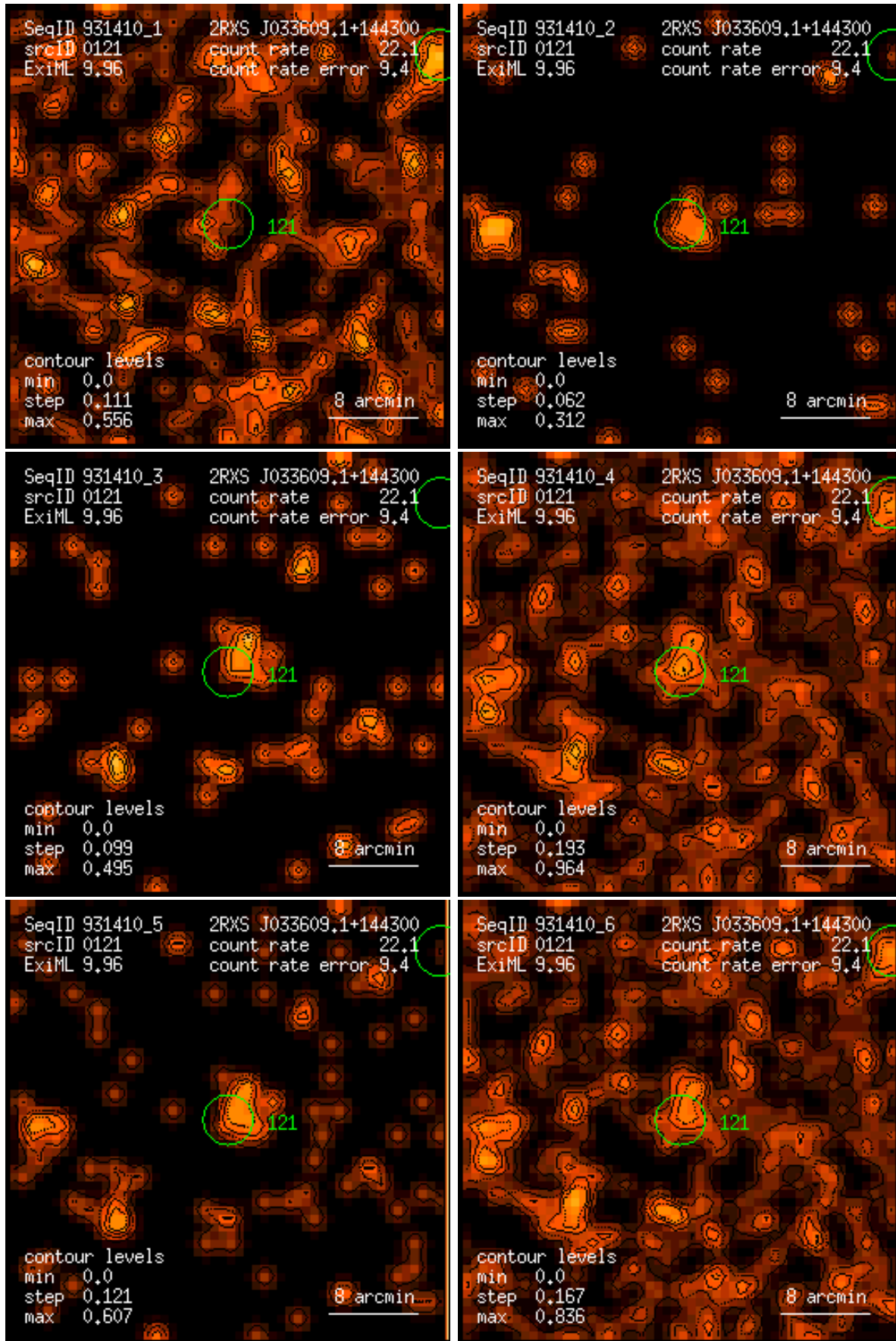
Figure 121: RASS 931410: detection 0121: band rate images, Gaussian filter: (1) PSPC channels 11 – 41, (2) 52 – 90, (3) 91 – 201, (4) 11 – 235, (5) 52 – 201, (6) 11 – 201. Broad band rates in counts/ks. Band rate contour levels in counts/ks/arcmin 2 .
