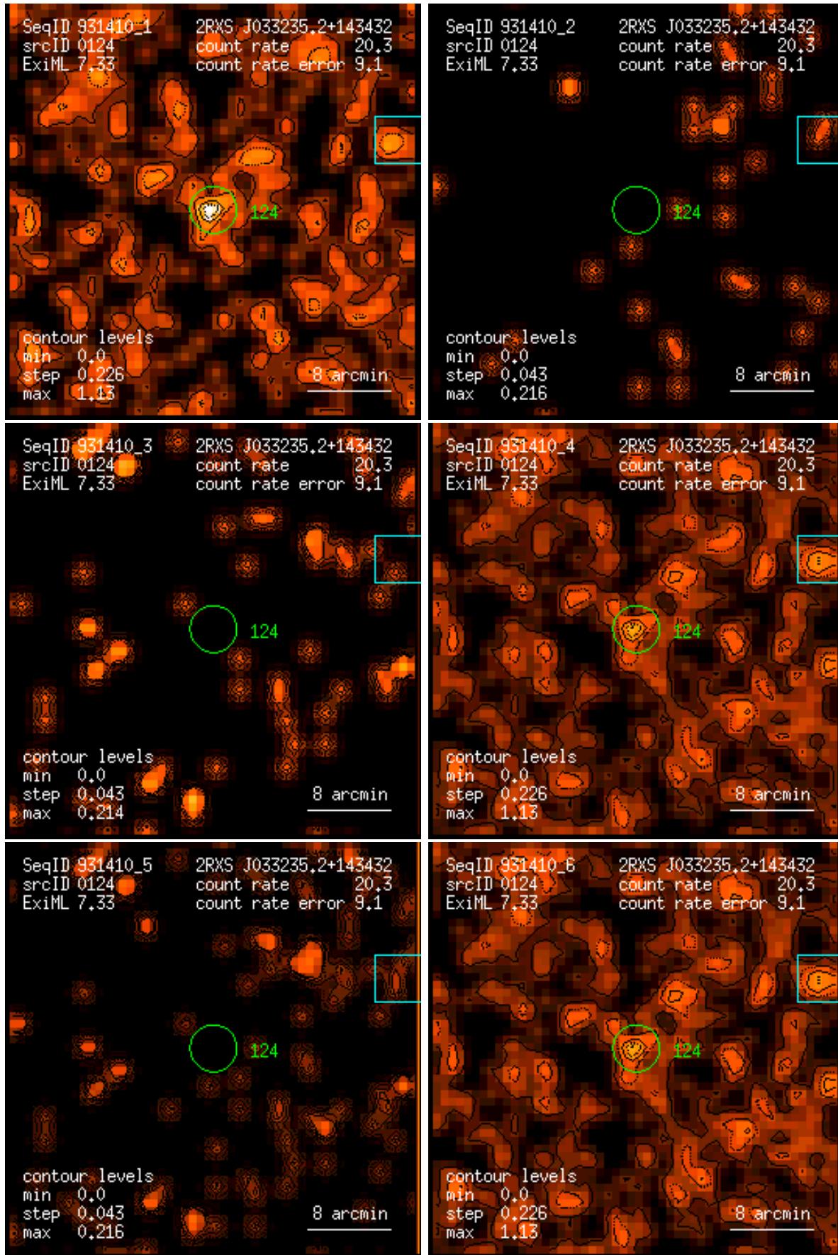
Figure 124: RASS 931410: detection 0124: band rate images, Gaussian filter: (1) PSPC channels 11 – 41, (2) 52 – 90, (3) 91 – 201, (4) 11 – 235, (5) 52 – 201, (6) 11 – 201. Broad band rates in counts/ks. Band rate contour levels in counts/ks/arcmin 2 .
