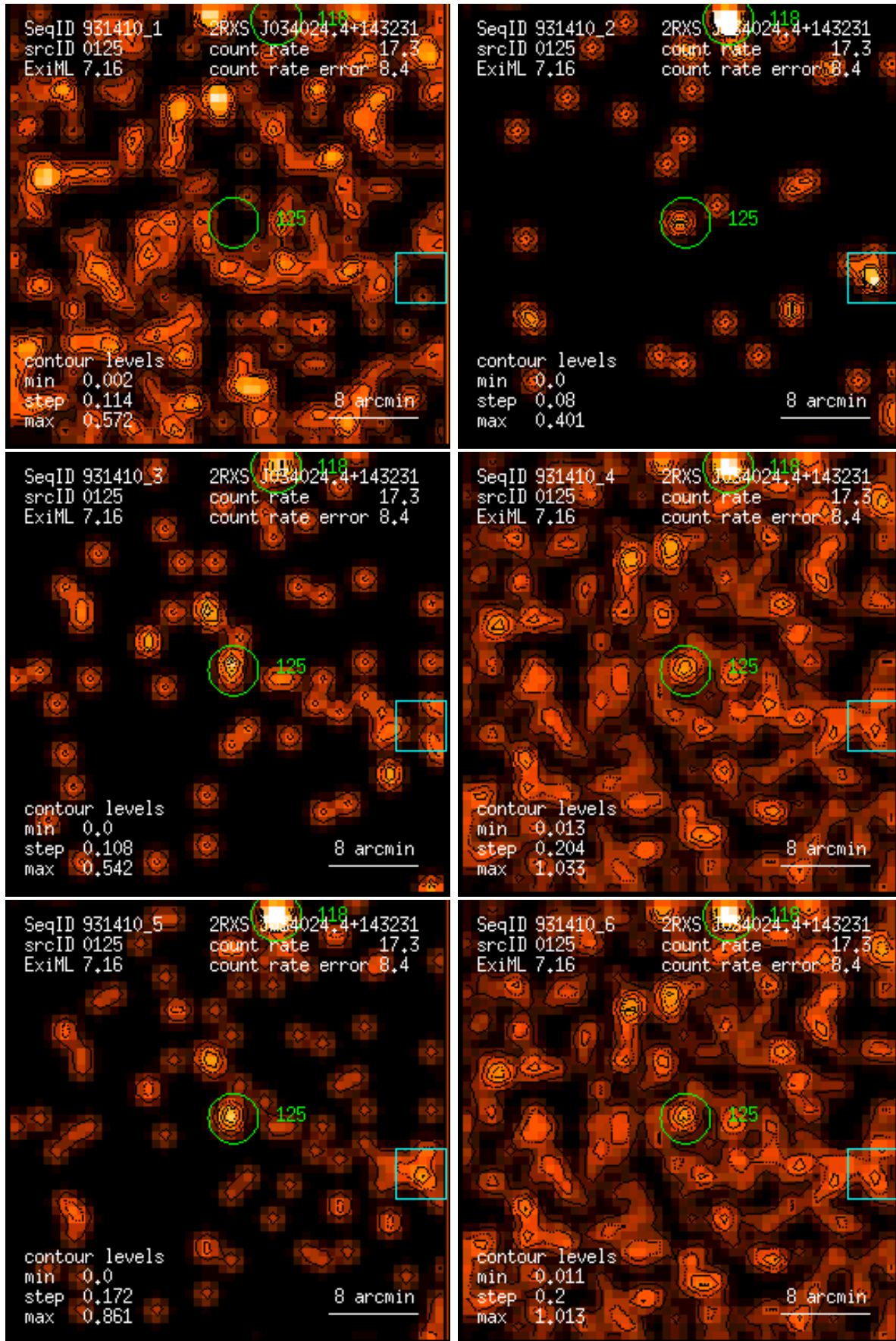
Figure 125: RASS 931410: detection 0125: band rate images, Gaussian filter: (1) PSPC channels 11 – 41, (2) 52 – 90, (3) 91 – 201, (4) 11 – 235, (5) 52 – 201, (6) 11 – 201. Broad band rates in counts/ks. Band rate contour levels in counts/ks/arcmin 2 .
