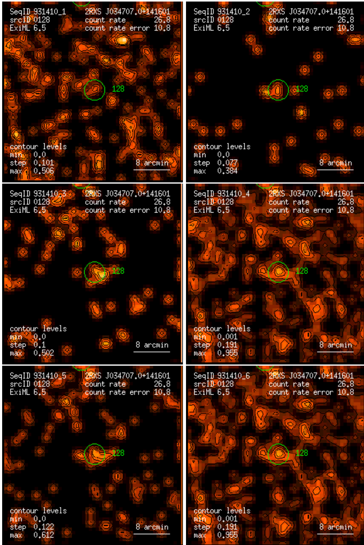
Figure 128: RASS 931410: detection 0128: band rate images, Gaussian filter: (1) PSPC channels 11 – 41, (2) 52 – 90, (3) 91 – 201, (4) 11 – 235, (5) 52 – 201, (6) 11 – 201. Broad band rates in counts/ks. Band rate contour levels in counts/ks/arcmin 2 .
