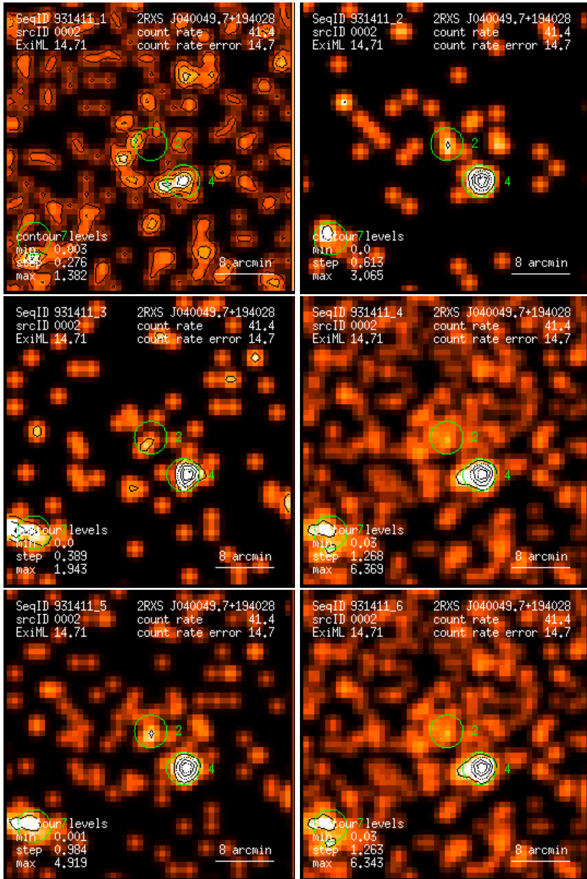
Figure 2: RASS 931411: detection 0002: band rate images, Gaussian filter: (1) PSPC channels 11 – 41, (2) 52 – 90, (3) 91 – 201, (4) 11 – 235, (5) 52 – 201, (6) 11 – 201. Broad band rates in counts/ks. Band rate contour levels in counts/ks/arcmin 2 .
