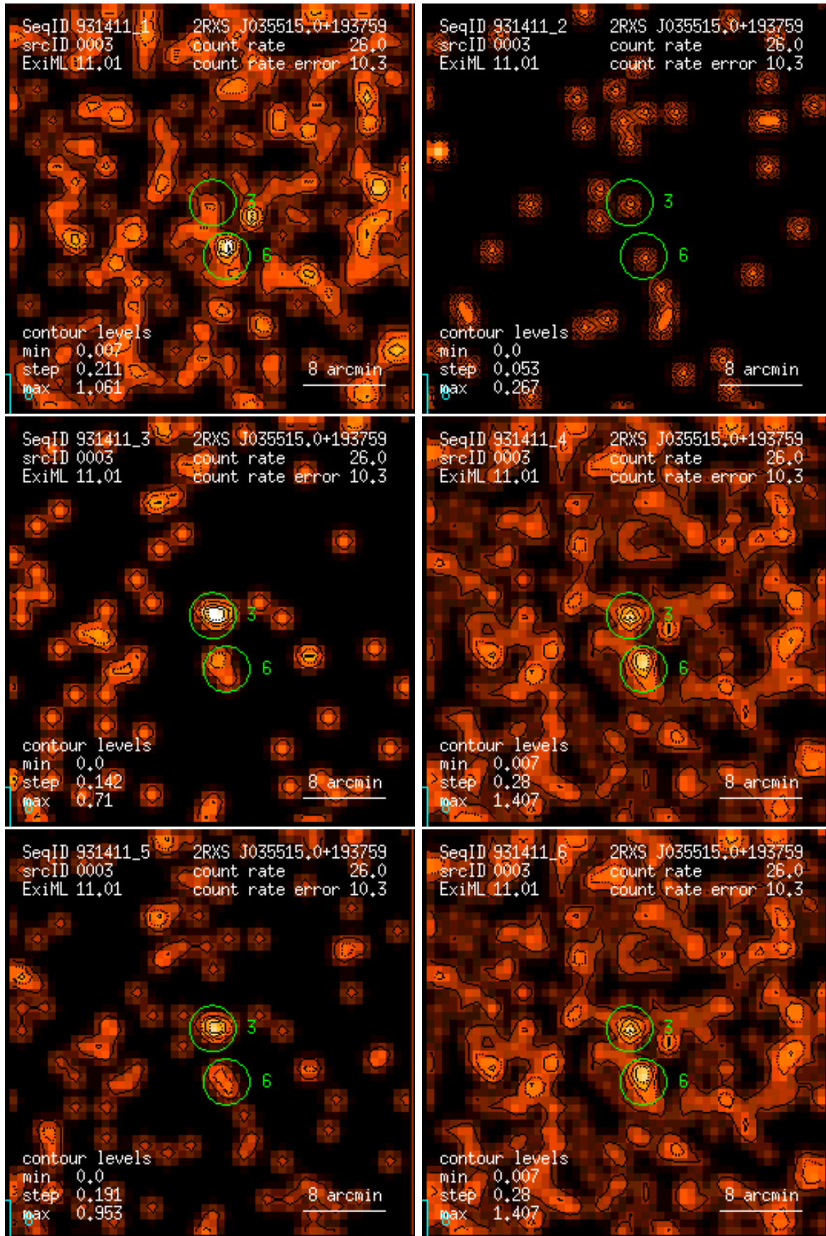
Figure 3: RASS 931411: detection 0003: band rate images, Gaussian filter: (1) PSPC channels 11 – 41, (2) 52 – 90, (3) 91 – 201, (4) 11 – 235, (5) 52 – 201, (6) 11 – 201. Broad band rates in counts/ks. Band rate contour levels in counts/ks/arcmin 2 .
