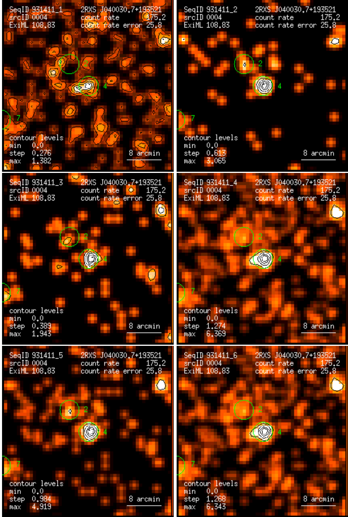
Figure 4: RASS 931411: detection 0004: band rate images, Gaussian filter: (1) PSPC channels 11 – 41, (2) 52 – 90, (3) 91 – 201, (4) 11 – 235, (5) 52 – 201, (6) 11 – 201. Broad band rates in counts/ks. Band rate contour levels in counts/ks/arcmin 2 .
