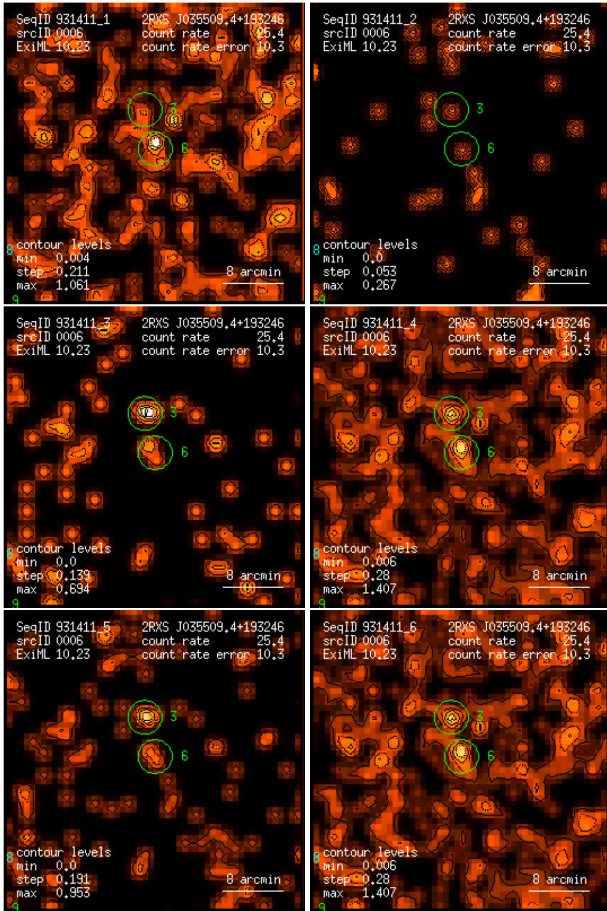
Figure 6: RASS 931411: detection 0006: band rate images, Gaussian filter: (1) PSPC channels 11 – 41, (2) 52 – 90, (3) 91 – 201, (4) 11 – 235, (5) 52 – 201, (6) 11 – 201. Broad band rates in counts/ks. Band rate contour levels in counts/ks/arcmin 2 .
