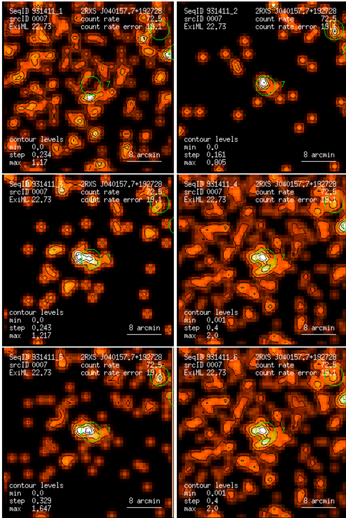
Figure 7: RASS 931411: detection 0007: band rate images, Gaussian filter: (1) PSPC channels 11 – 41, (2) 52 – 90, (3) 91 – 201, (4) 11 – 235, (5) 52 – 201, (6) 11 – 201. Broad band rates in counts/ks. Band rate contour levels in counts/ks/arcmin 2 .
