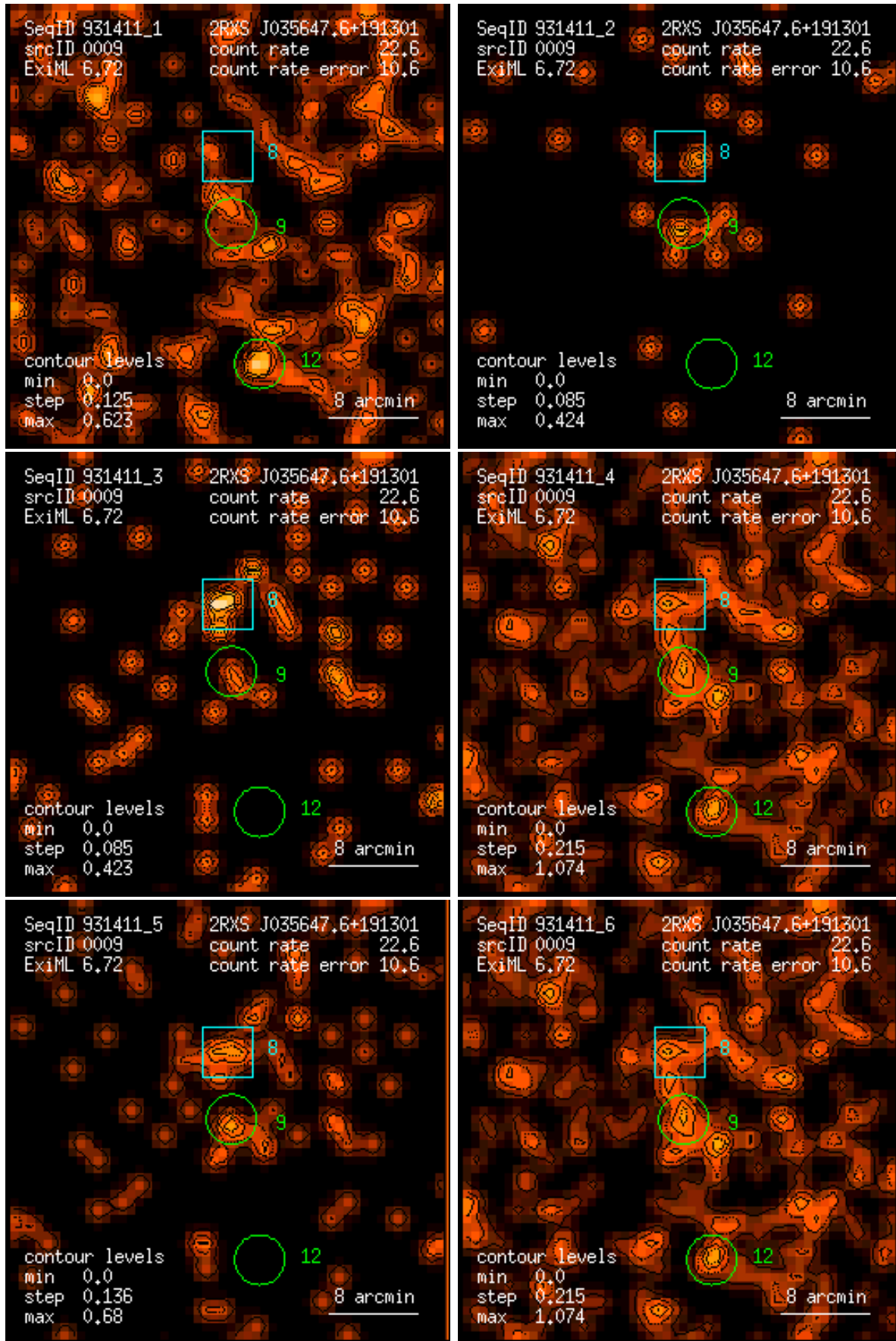
Figure 9: RASS 931411: detection 0009: band rate images, Gaussian filter: (1) PSPC channels 11 – 41, (2) 52 – 90, (3) 91 – 201, (4) 11 – 235, (5) 52 – 201, (6) 11 – 201. Broad band rates in counts/ks. Band rate contour levels in counts/ks/arcmin 2 .
