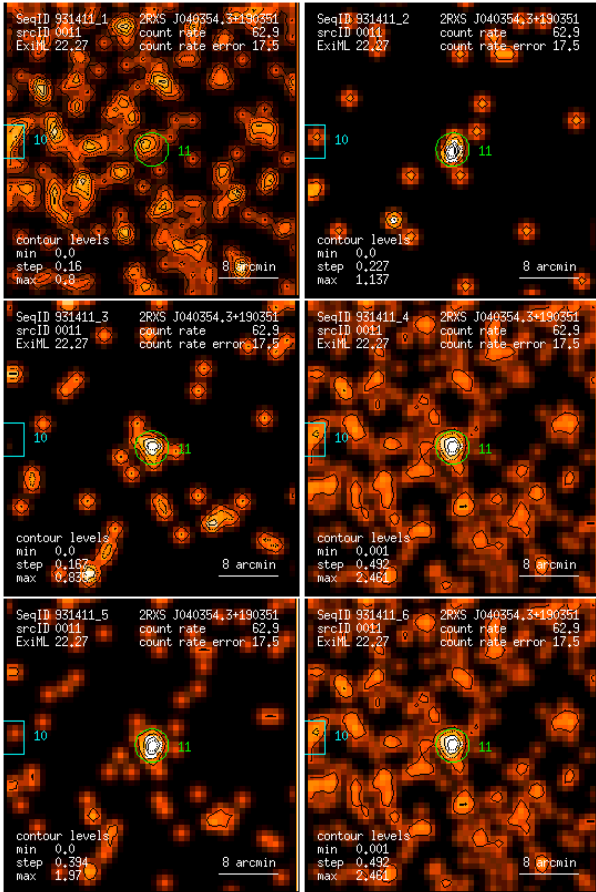
Figure 11: RASS 931411: detection 0011: band rate images, Gaussian filter: (1) PSPC channels 11 – 41, (2) 52 – 90, (3) 91 – 201, (4) 11 – 235, (5) 52 – 201, (6) 11 – 201. Broad band rates in counts/ks. Band rate contour levels in counts/ks/arcmin 2 .
