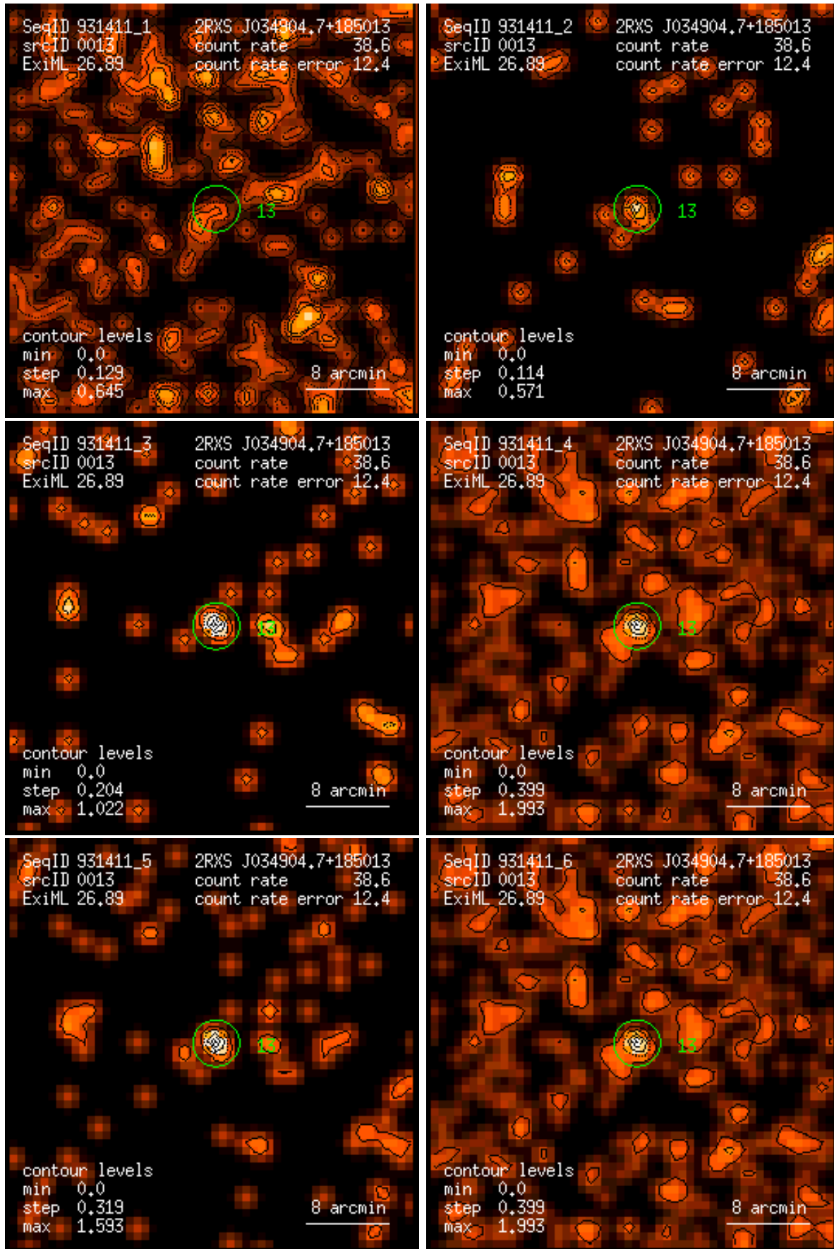
Figure 13: RASS 931411: detection 0013: band rate images, Gaussian filter: (1) PSPC channels 11 – 41, (2) 52 – 90, (3) 91 – 201, (4) 11 – 235, (5) 52 – 201, (6) 11 – 201. Broad band rates in counts/ks. Band rate contour levels in counts/ks/arcmin 2 .
