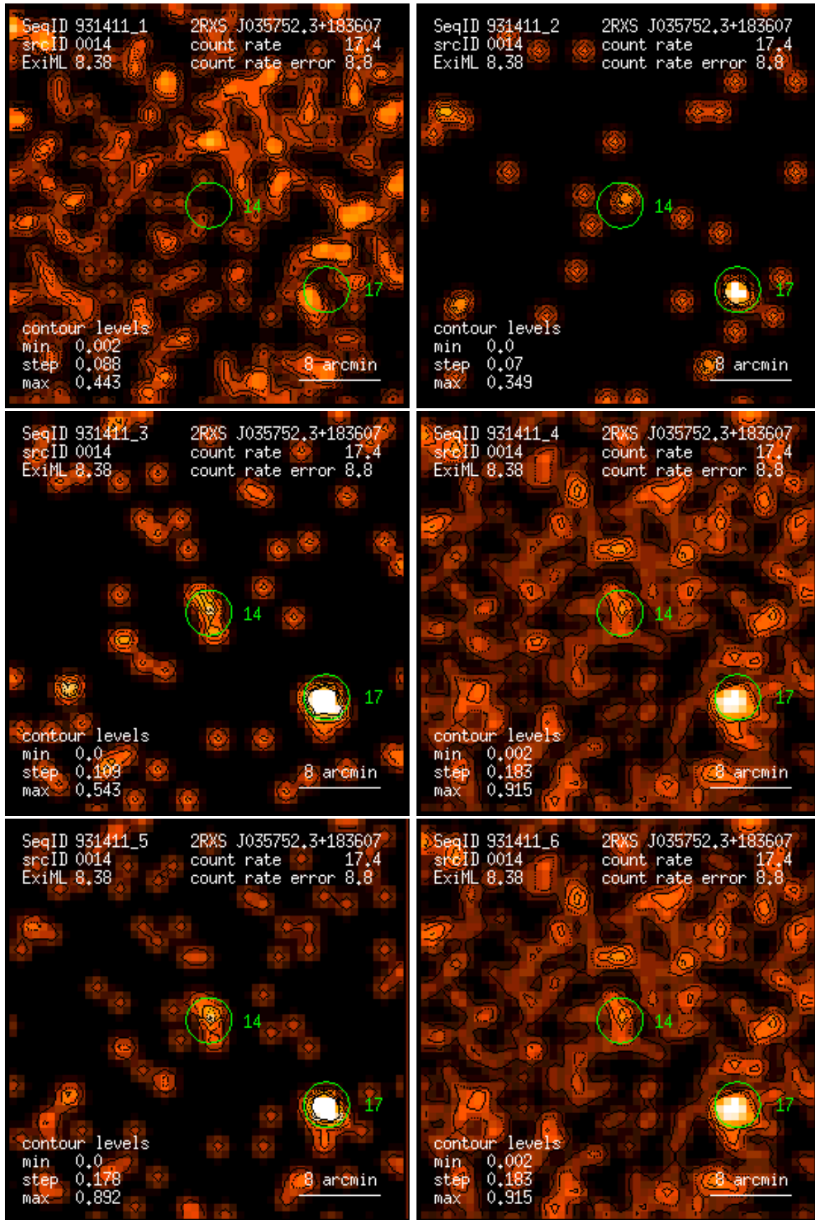
Figure 14: RASS 931411: detection 0014: band rate images, Gaussian filter: (1) PSPC channels 11 – 41, (2) 52 – 90, (3) 91 – 201, (4) 11 – 235, (5) 52 – 201, (6) 11 – 201. Broad band rates in counts/ks. Band rate contour levels in counts/ks/arcmin 2 .
