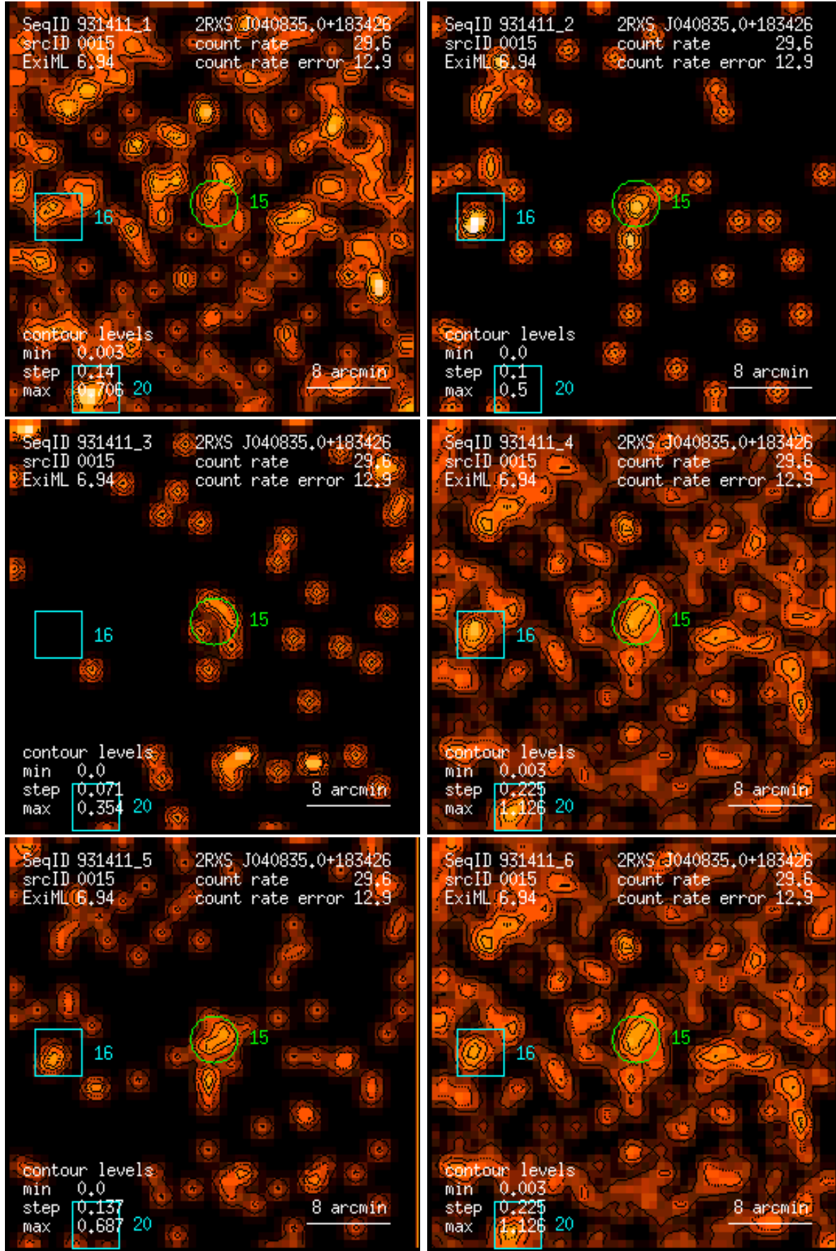
Figure 15: RASS 931411: detection 0015: band rate images, Gaussian filter: (1) PSPC channels 11 – 41, (2) 52 – 90, (3) 91 – 201, (4) 11 – 235, (5) 52 – 201, (6) 11 – 201. Broad band rates in counts/ks. Band rate contour levels in counts/ks/arcmin 2 .
