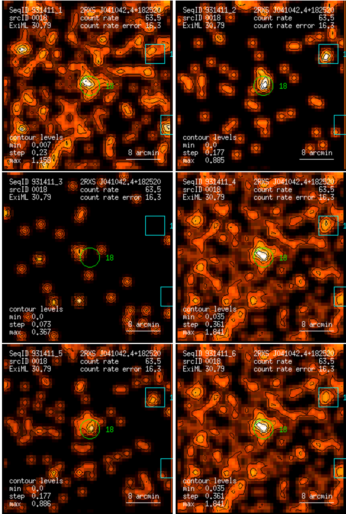
Figure 18: RASS 931411: detection 0018: band rate images, Gaussian filter: (1) PSPC channels 11 – 41, (2) 52 – 90, (3) 91 – 201, (4) 11 – 235, (5) 52 – 201, (6) 11 – 201. Broad band rates in counts/ks. Band rate contour levels in counts/ks/arcmin 2 .
