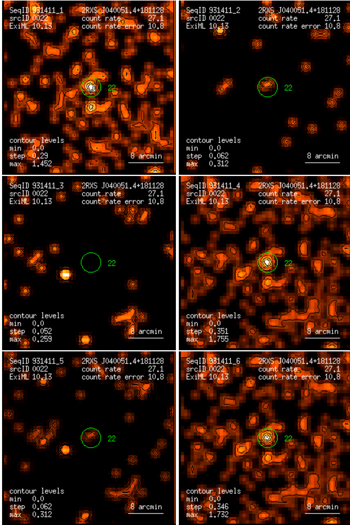
Figure 22: RASS 931411: detection 0022: band rate images, Gaussian filter: (1) PSPC channels 11 – 41, (2) 52 – 90, (3) 91 – 201, (4) 11 – 235, (5) 52 – 201, (6) 11 – 201. Broad band rates in counts/ks. Band rate contour levels in counts/ks/arcmin 2 .
