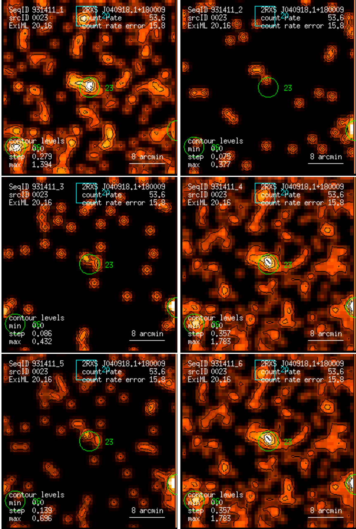
Figure 23: RASS 931411: detection 0023: band rate images, Gaussian filter: (1) PSPC channels 11 – 41, (2) 52 – 90, (3) 91 – 201, (4) 11 – 235, (5) 52 – 201, (6) 11 – 201. Broad band rates in counts/ks. Band rate contour levels in counts/ks/arcmin 2 .
