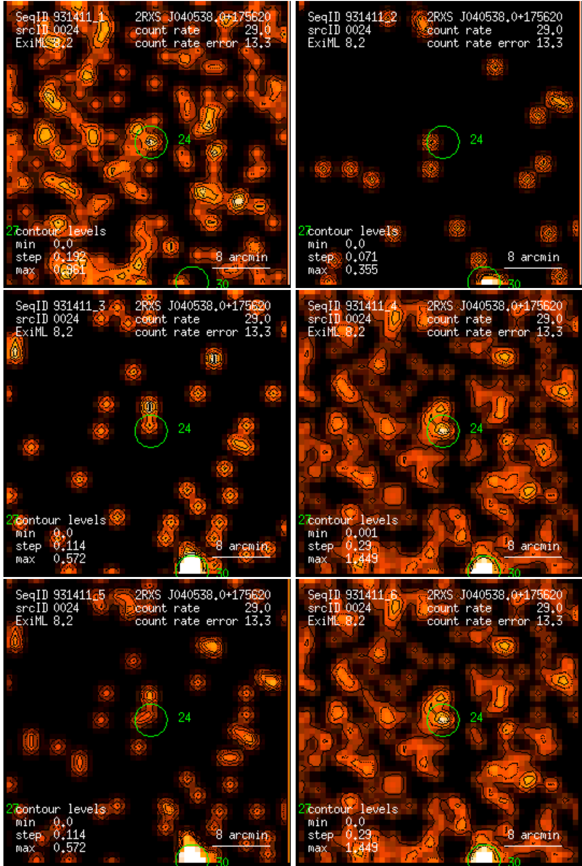
Figure 24: RASS 931411: detection 0024: band rate images, Gaussian filter: (1) PSPC channels 11 – 41, (2) 52 – 90, (3) 91 – 201, (4) 11 – 235, (5) 52 – 201, (6) 11 – 201. Broad band rates in counts/ks. Band rate contour levels in counts/ks/arcmin 2 .
