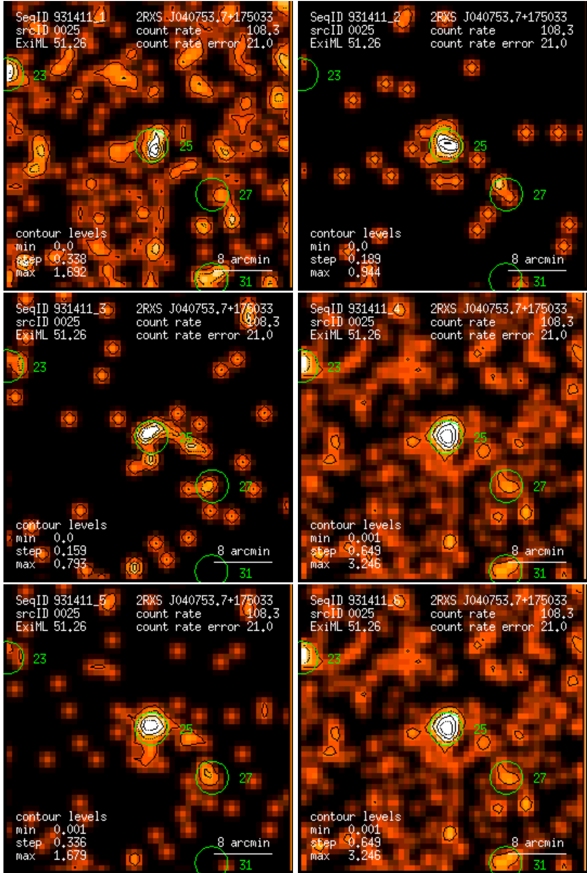
Figure 25: RASS 931411: detection 0025: band rate images, Gaussian filter: (1) PSPC channels 11 – 41, (2) 52 – 90, (3) 91 – 201, (4) 11 – 235, (5) 52 – 201, (6) 11 – 201. Broad band rates in counts/ks. Band rate contour levels in counts/ks/arcmin 2 .
