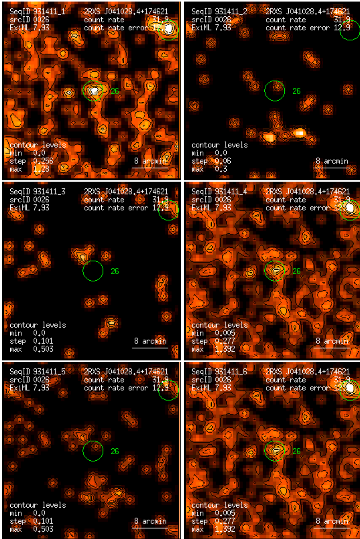
Figure 26: RASS 931411: detection 0026: band rate images, Gaussian filter: (1) PSPC channels 11 – 41, (2) 52 – 90, (3) 91 – 201, (4) 11 – 235, (5) 52 – 201, (6) 11 – 201. Broad band rates in counts/ks. Band rate contour levels in counts/ks/arcmin 2 .
