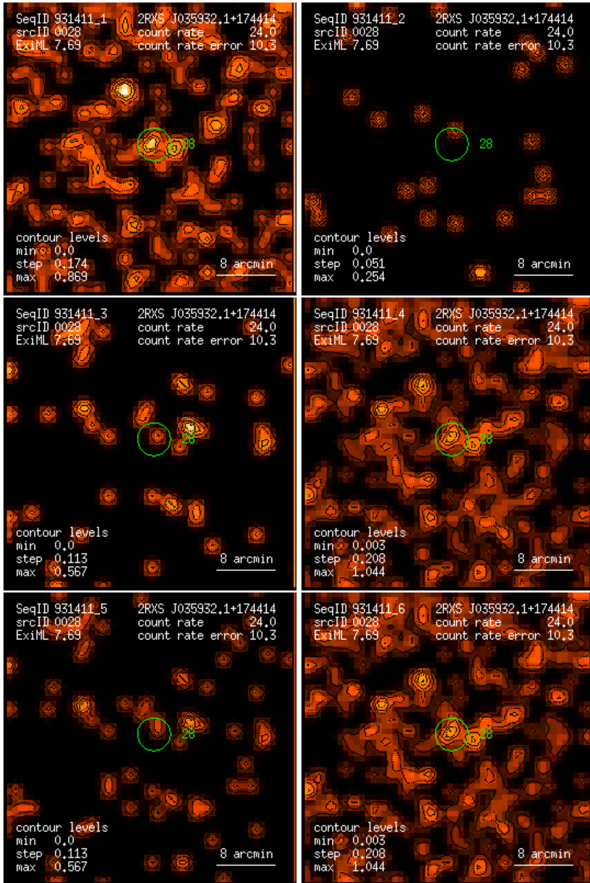
Figure 28: RASS 931411: detection 0028: band rate images, Gaussian filter: (1) PSPC channels 11 – 41, (2) 52 – 90, (3) 91 – 201, (4) 11 – 235, (5) 52 – 201, (6) 11 – 201. Broad band rates in counts/ks. Band rate contour levels in counts/ks/arcmin 2 .
