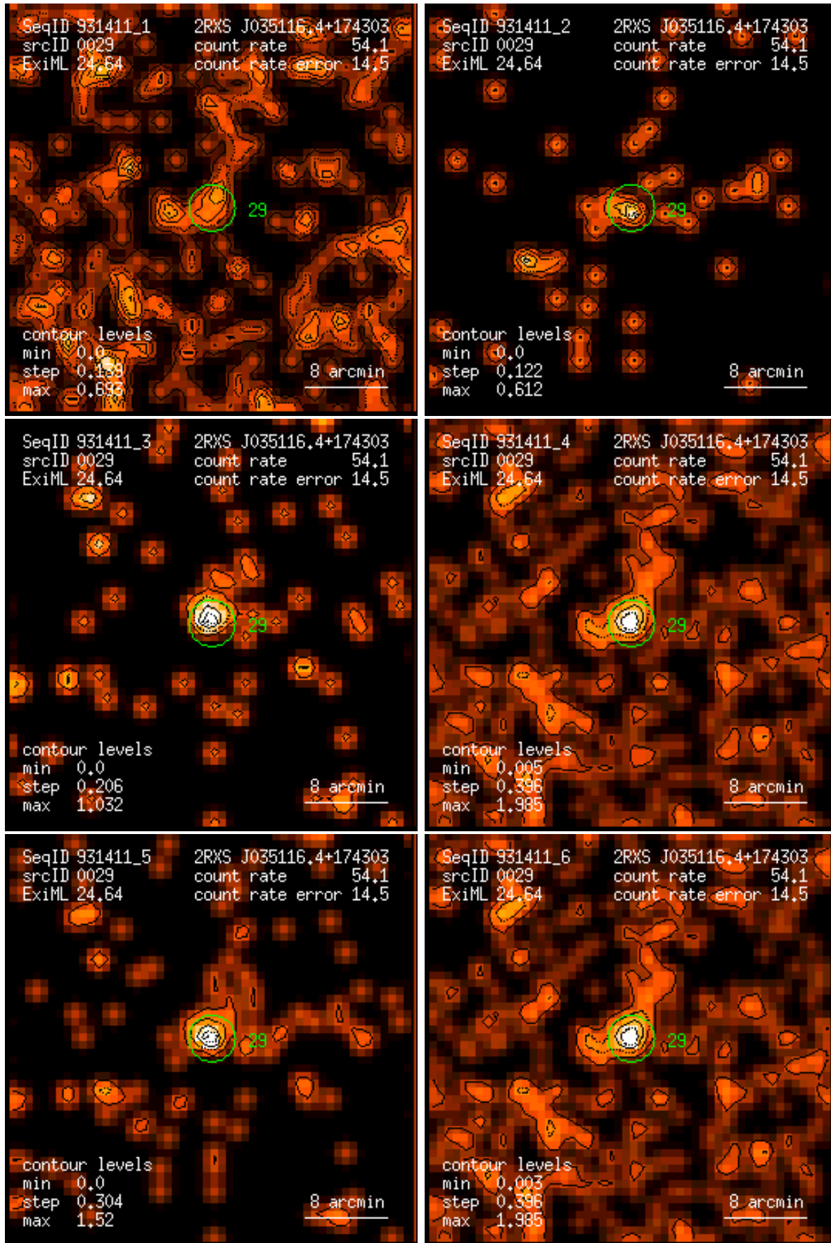
Figure 29: RASS 931411: detection 0029: band rate images, Gaussian filter: (1) PSPC channels 11 – 41, (2) 52 – 90, (3) 91 – 201, (4) 11 – 235, (5) 52 – 201, (6) 11 – 201. Broad band rates in counts/ks. Band rate contour levels in counts/ks/arcmin 2 .
