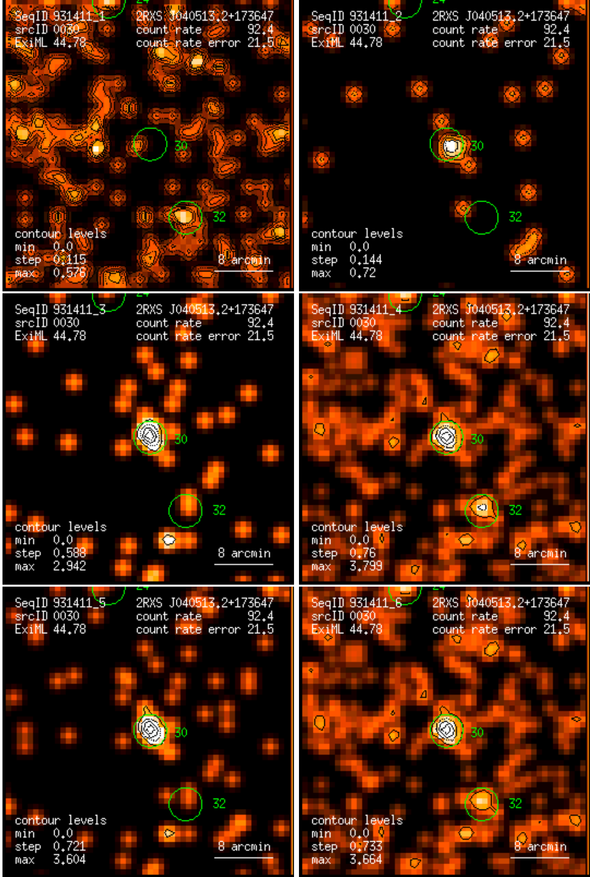
Figure 30: RASS 931411: detection 0030: band rate images, Gaussian filter: (1) PSPC channels 11 – 41, (2) 52 – 90, (3) 91 – 201, (4) 11 – 235, (5) 52 – 201, (6) 11 – 201. Broad band rates in counts/ks. Band rate contour levels in counts/ks/arcmin 2 .
