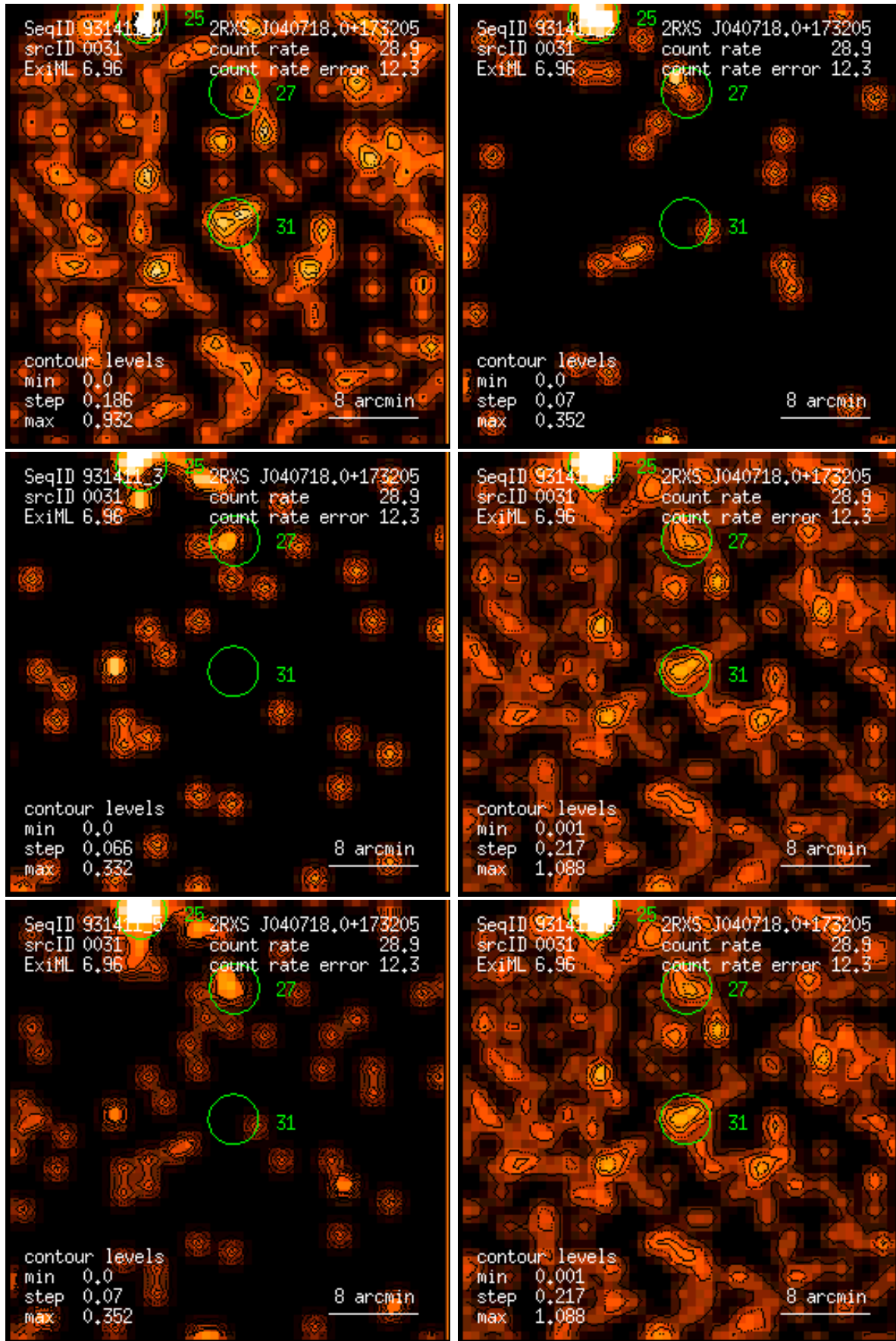
Figure 31: RASS 931411: detection 0031: band rate images, Gaussian filter: (1) PSPC channels 11 – 41, (2) 52 – 90, (3) 91 – 201, (4) 11 – 235, (5) 52 – 201, (6) 11 – 201. Broad band rates in counts/ks. Band rate contour levels in counts/ks/arcmin 2 .
