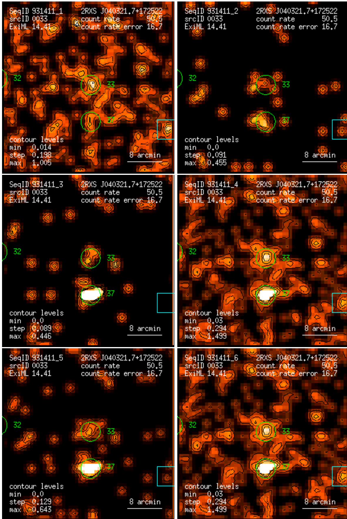
Figure 33: RASS 931411: detection 0033: band rate images, Gaussian filter: (1) PSPC channels 11 – 41, (2) 52 – 90, (3) 91 – 201, (4) 11 – 235, (5) 52 – 201, (6) 11 – 201. Broad band rates in counts/ks. Band rate contour levels in counts/ks/arcmin 2 .
