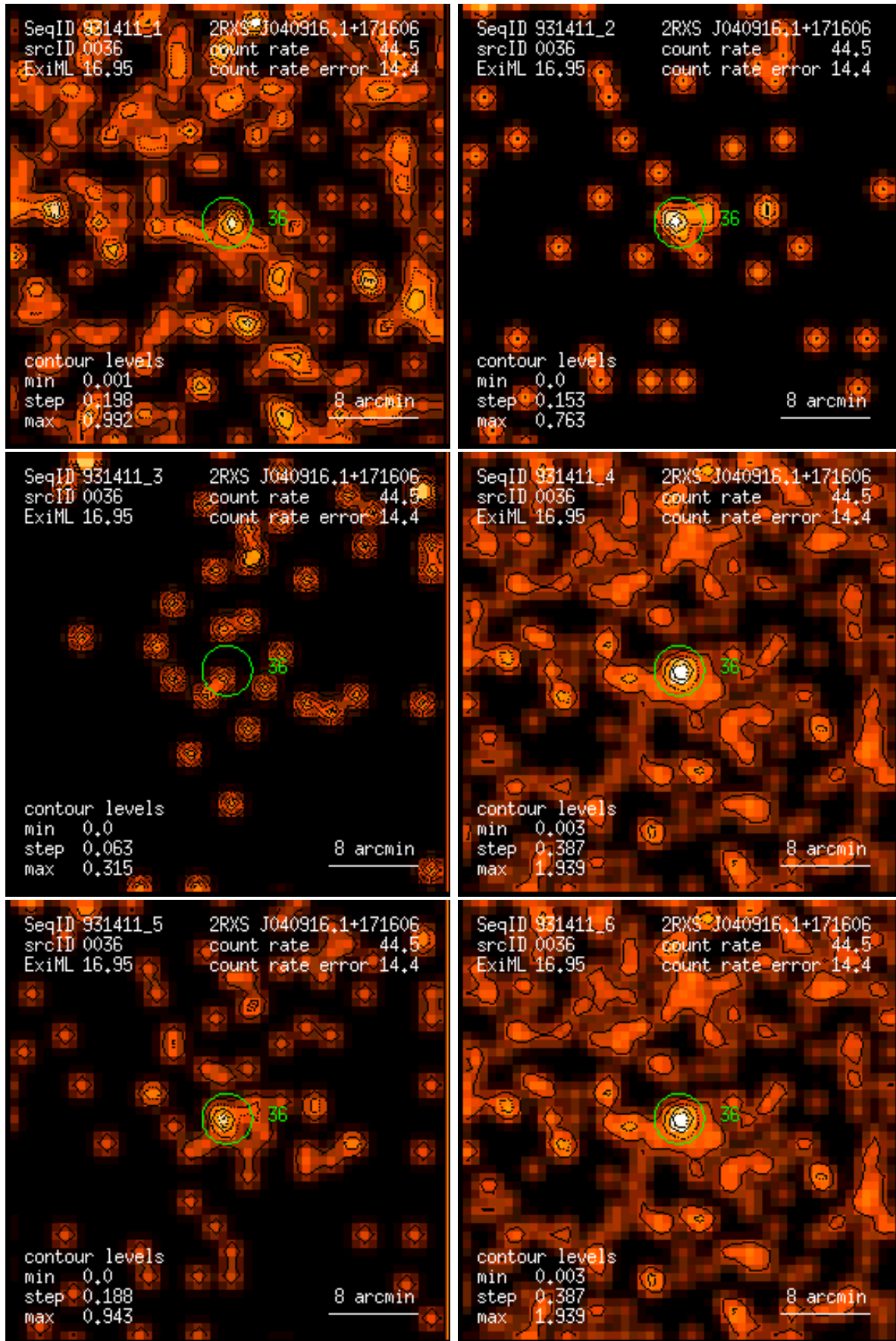
Figure 36: RASS 931411: detection 0036: band rate images, Gaussian filter: (1) PSPC channels 11 – 41, (2) 52 – 90, (3) 91 – 201, (4) 11 – 235, (5) 52 – 201, (6) 11 – 201. Broad band rates in counts/ks. Band rate contour levels in counts/ks/arcmin 2 .
