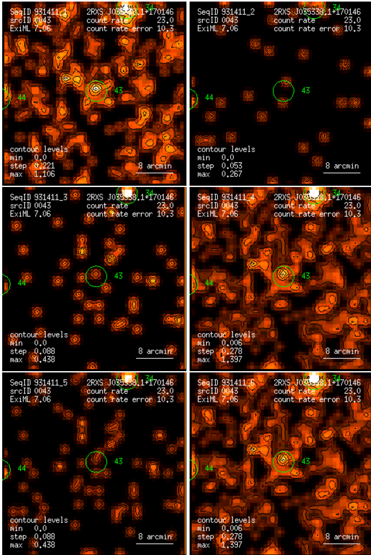
Figure 43: RASS 931411: detection 0043: band rate images, Gaussian filter: (1) PSPC channels 11 – 41, (2) 52 – 90, (3) 91 – 201, (4) 11 – 235, (5) 52 – 201, (6) 11 – 201. Broad band rates in counts/ks. Band rate contour levels in counts/ks/arcmin 2 .
