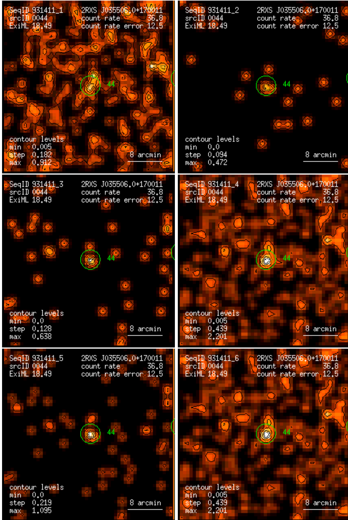
Figure 44: RASS 931411: detection 0044: band rate images, Gaussian filter: (1) PSPC channels 11 – 41, (2) 52 – 90, (3) 91 – 201, (4) 11 – 235, (5) 52 – 201, (6) 11 – 201. Broad band rates in counts/ks. Band rate contour levels in counts/ks/arcmin 2 .
