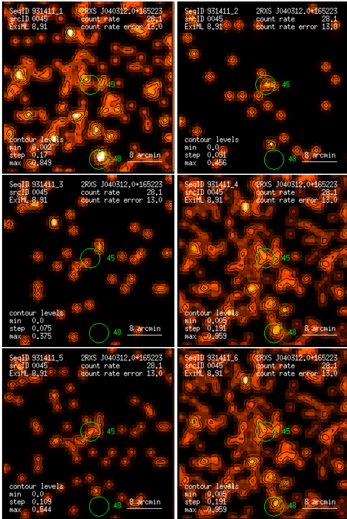
Figure 45: RASS 931411: detection 0045: band rate images, Gaussian filter: (1) PSPC channels 11 – 41, (2) 52 – 90, (3) 91 – 201, (4) 11 – 235, (5) 52 – 201, (6) 11 – 201. Broad band rates in counts/ks. Band rate contour levels in counts/ks/arcmin 2 .
