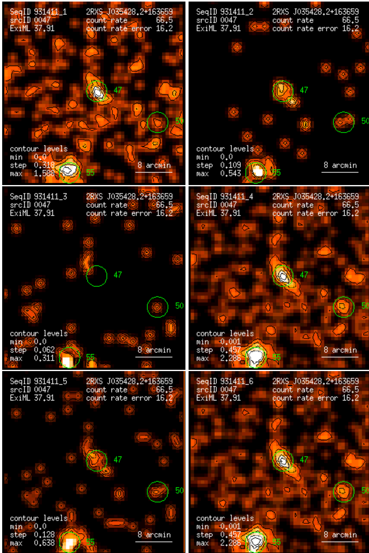
Figure 47: RASS 931411: detection 0047: band rate images, Gaussian filter: (1) PSPC channels 11 – 41, (2) 52 – 90, (3) 91 – 201, (4) 11 – 235, (5) 52 – 201, (6) 11 – 201. Broad band rates in counts/ks. Band rate contour levels in counts/ks/arcmin 2 .
