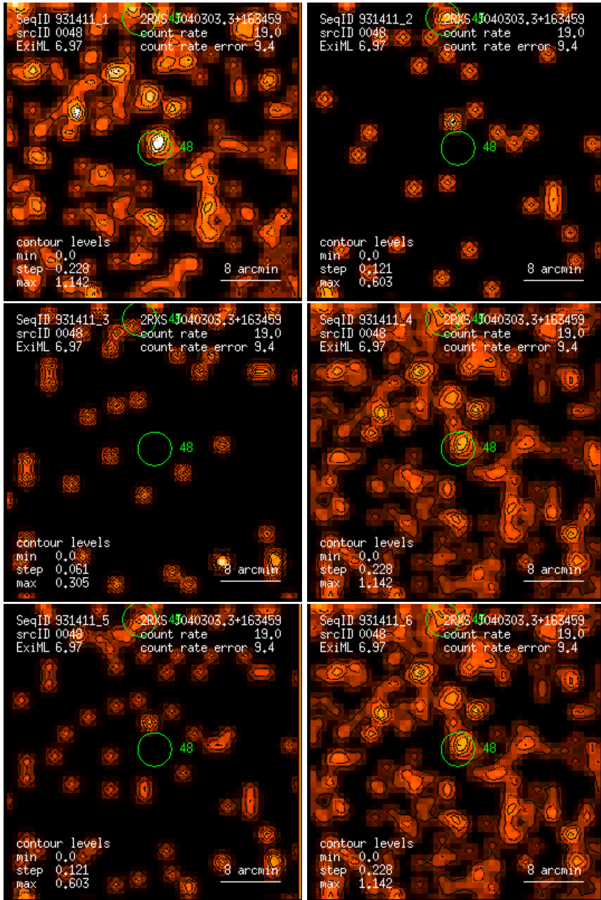
Figure 48: RASS 931411: detection 0048: band rate images, Gaussian filter: (1) PSPC channels 11 – 41, (2) 52 – 90, (3) 91 – 201, (4) 11 – 235, (5) 52 – 201, (6) 11 – 201. Broad band rates in counts/ks. Band rate contour levels in counts/ks/arcmin 2 .
