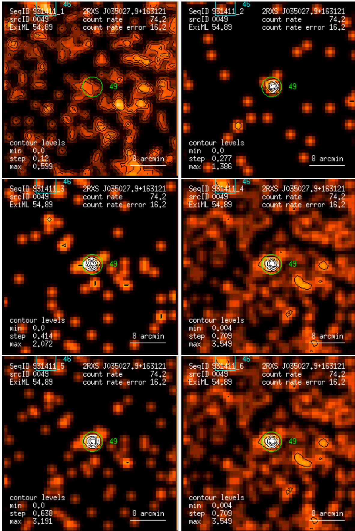
Figure 49: RASS 931411: detection 0049: band rate images, Gaussian filter: (1) PSPC channels 11 – 41, (2) 52 – 90, (3) 91 – 201, (4) 11 – 235, (5) 52 – 201, (6) 11 – 201. Broad band rates in counts/ks. Band rate contour levels in counts/ks/arcmin 2 .
