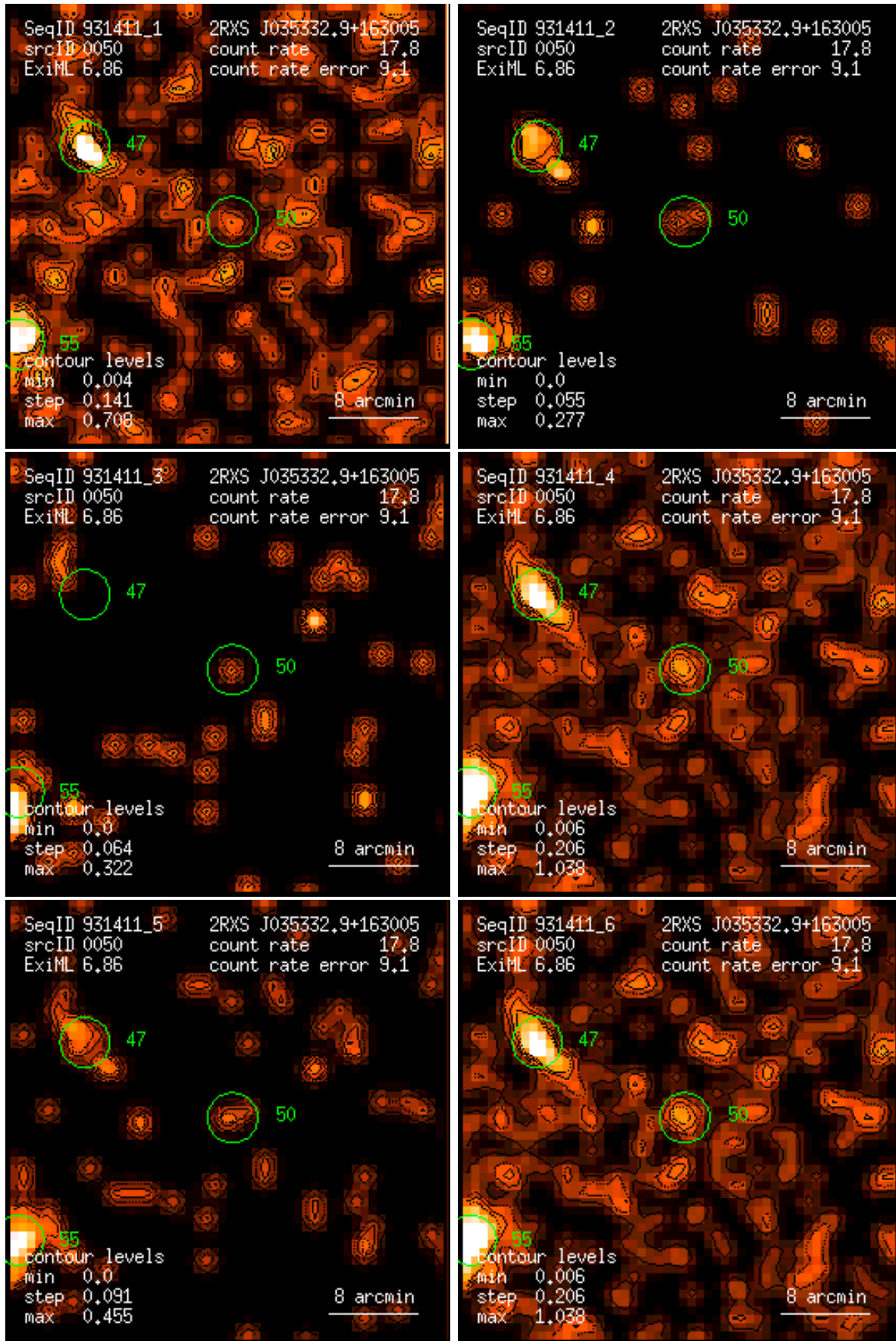
Figure 50: RASS 931411: detection 0050: band rate images, Gaussian filter: (1) PSPC channels 11 – 41, (2) 52 – 90, (3) 91 – 201, (4) 11 – 235, (5) 52 – 201, (6) 11 – 201. Broad band rates in counts/ks. Band rate contour levels in counts/ks/arcmin 2 .
