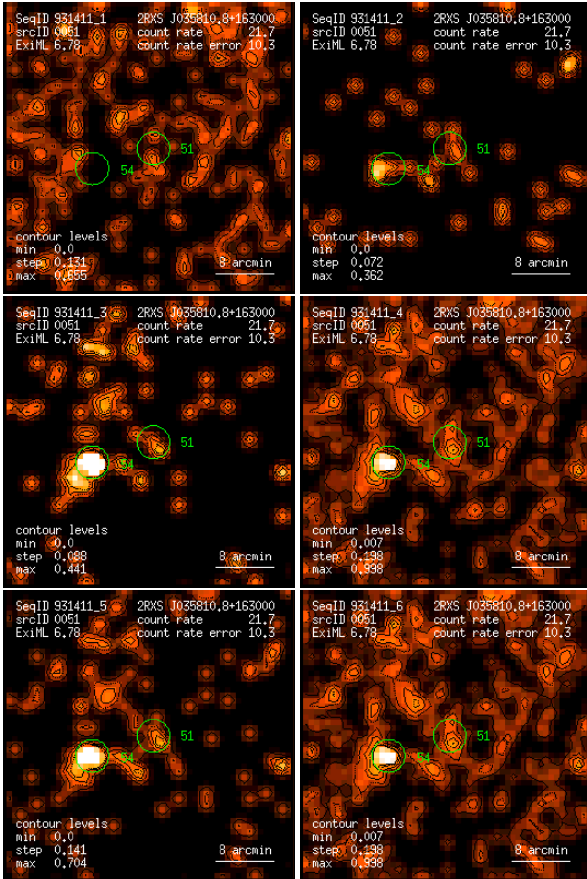
Figure 51: RASS 931411: detection 0051: band rate images, Gaussian filter: (1) PSPC channels 11 – 41, (2) 52 – 90, (3) 91 – 201, (4) 11 – 235, (5) 52 – 201, (6) 11 – 201. Broad band rates in counts/ks. Band rate contour levels in counts/ks/arcmin 2 .
