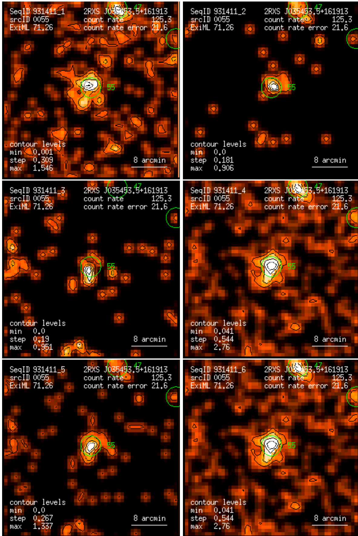
Figure 55: RASS 931411: detection 0055: band rate images, Gaussian filter: (1) PSPC channels 11 – 41, (2) 52 – 90, (3) 91 – 201, (4) 11 – 235, (5) 52 – 201, (6) 11 – 201. Broad band rates in counts/ks. Band rate contour levels in counts/ks/arcmin 2 .
