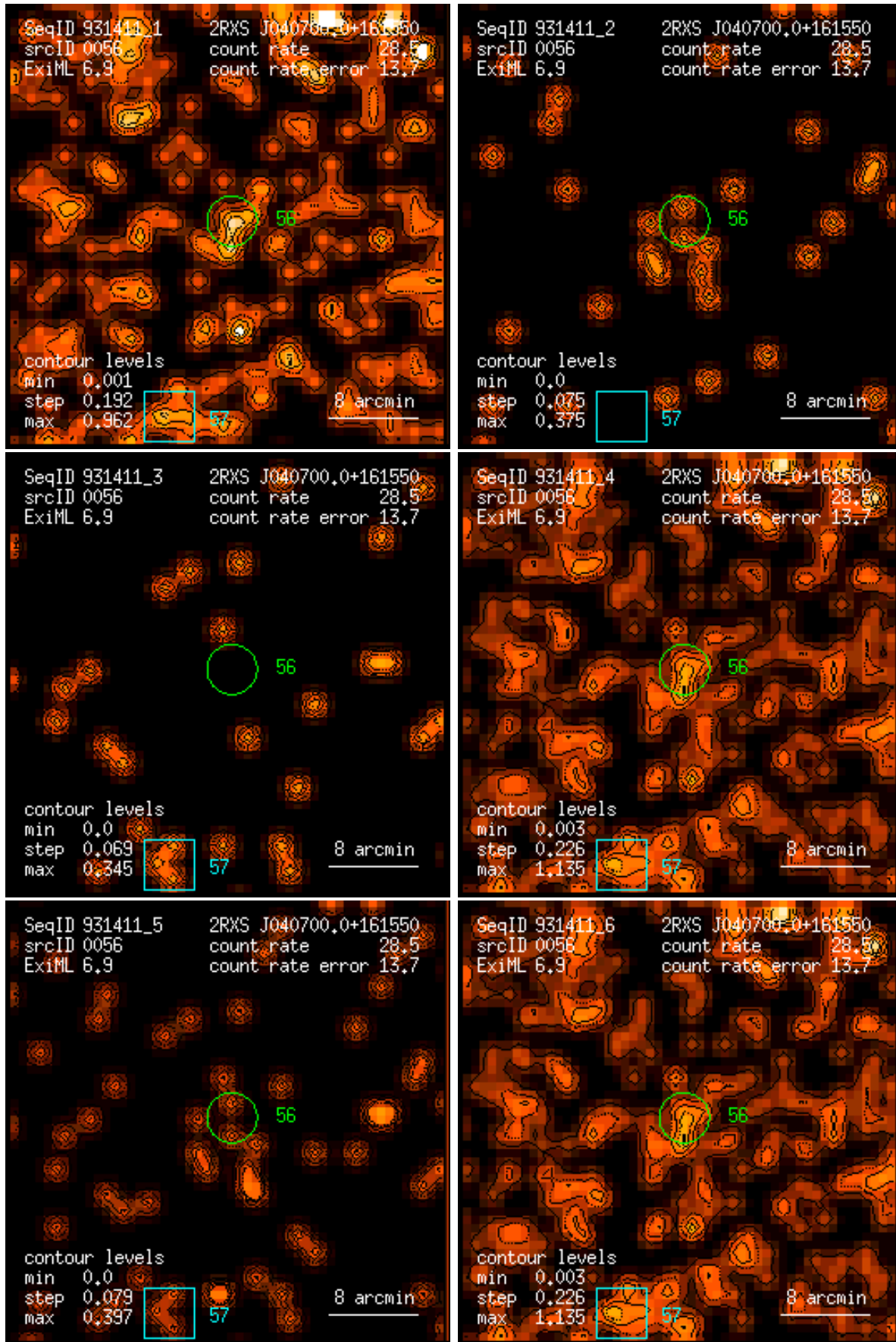
Figure 56: RASS 931411: detection 0056: band rate images, Gaussian filter: (1) PSPC channels 11 – 41, (2) 52 – 90, (3) 91 – 201, (4) 11 – 235, (5) 52 – 201, (6) 11 – 201. Broad band rates in counts/ks. Band rate contour levels in counts/ks/arcmin 2 .
