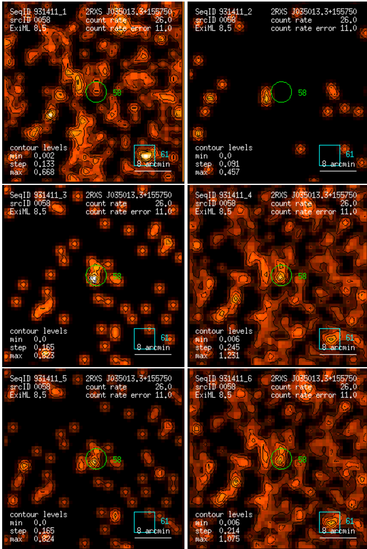
Figure 58: RASS 931411: detection 0058: band rate images, Gaussian filter: (1) PSPC channels 11 – 41, (2) 52 – 90, (3) 91 – 201, (4) 11 – 235, (5) 52 – 201, (6) 11 – 201. Broad band rates in counts/ks. Band rate contour levels in counts/ks/arcmin 2 .
