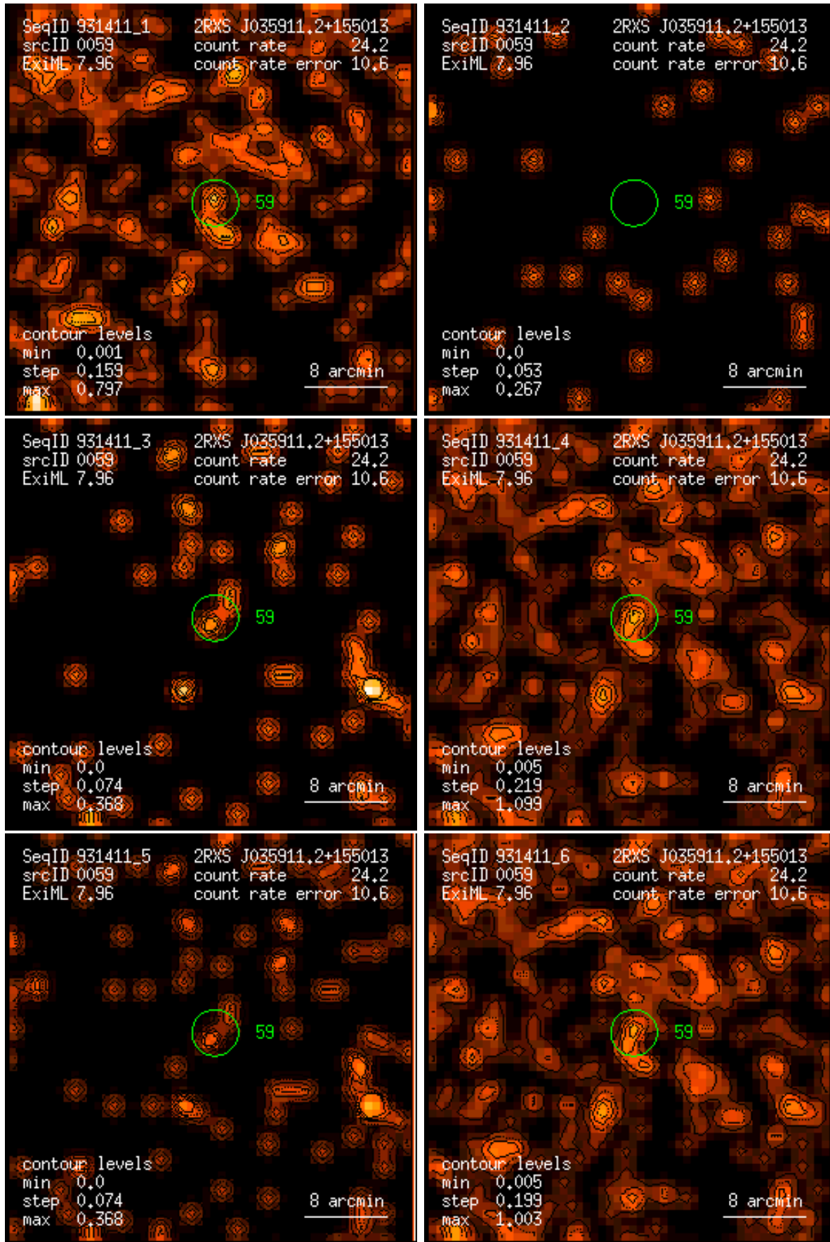
Figure 59: RASS 931411: detection 0059: band rate images, Gaussian filter: (1) PSPC channels 11 – 41, (2) 52 – 90, (3) 91 – 201, (4) 11 – 235, (5) 52 – 201, (6) 11 – 201. Broad band rates in counts/ks. Band rate contour levels in counts/ks/arcmin 2 .
