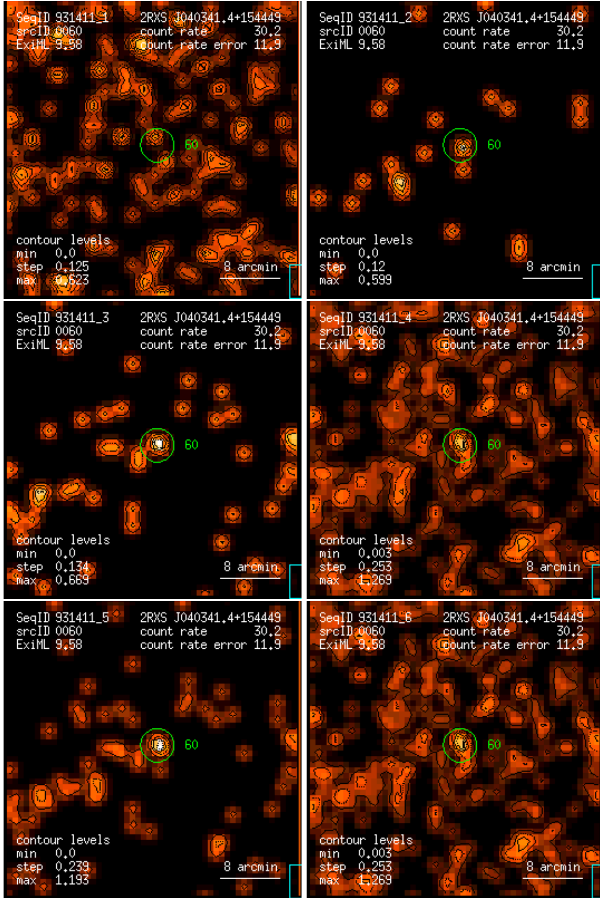
Figure 60: RASS 931411: detection 0060: band rate images, Gaussian filter: (1) PSPC channels 11 – 41, (2) 52 – 90, (3) 91 – 201, (4) 11 – 235, (5) 52 – 201, (6) 11 – 201. Broad band rates in counts/ks. Band rate contour levels in counts/ks/arcmin 2 .
