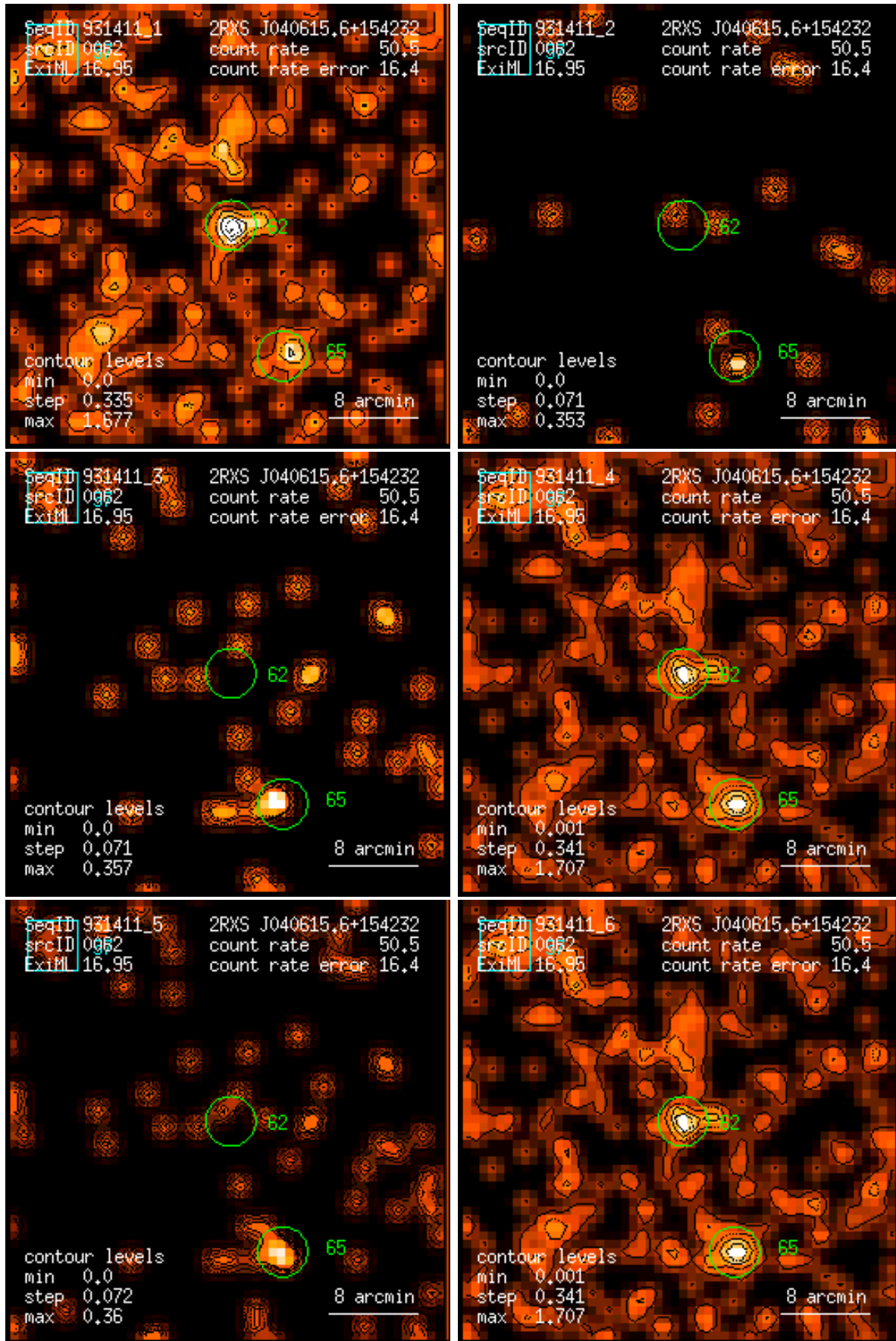
Figure 62: RASS 931411: detection 0062: band rate images, Gaussian filter: (1) PSPC channels 11 – 41, (2) 52 – 90, (3) 91 – 201, (4) 11 – 235, (5) 52 – 201, (6) 11 – 201. Broad band rates in counts/ks. Band rate contour levels in counts/ks/arcmin 2 .
