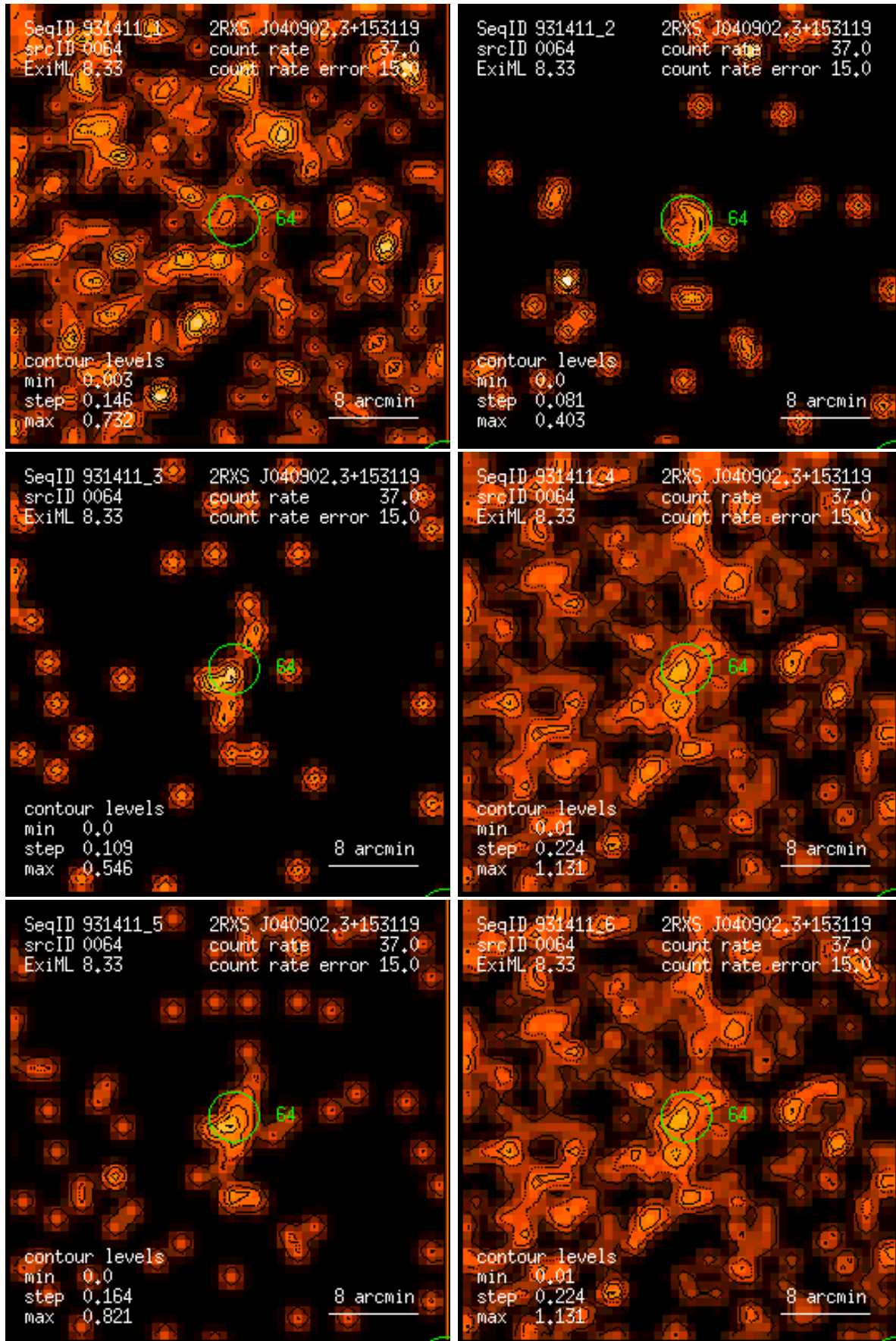
Figure 64: RASS 931411: detection 0064: band rate images, Gaussian filter: (1) PSPC channels 11 – 41, (2) 52 – 90, (3) 91 – 201, (4) 11 – 235, (5) 52 – 201, (6) 11 – 201. Broad band rates in counts/ks. Band rate contour levels in counts/ks/arcmin 2 .
