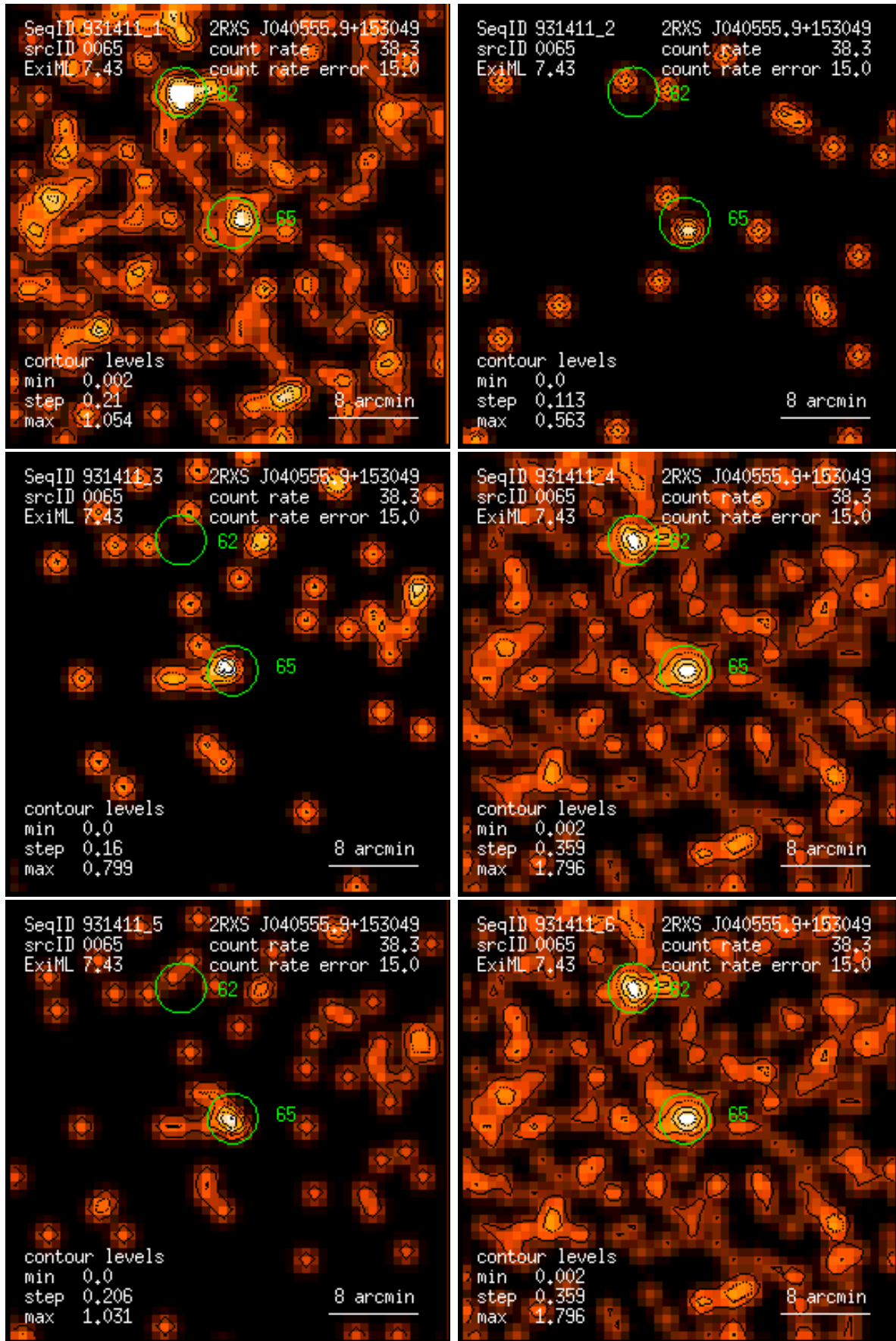
Figure 65: RASS 931411: detection 0065: band rate images, Gaussian filter: (1) PSPC channels 11 – 41, (2) 52 – 90, (3) 91 – 201, (4) 11 – 235, (5) 52 – 201, (6) 11 – 201. Broad band rates in counts/ks. Band rate contour levels in counts/ks/arcmin 2 .
