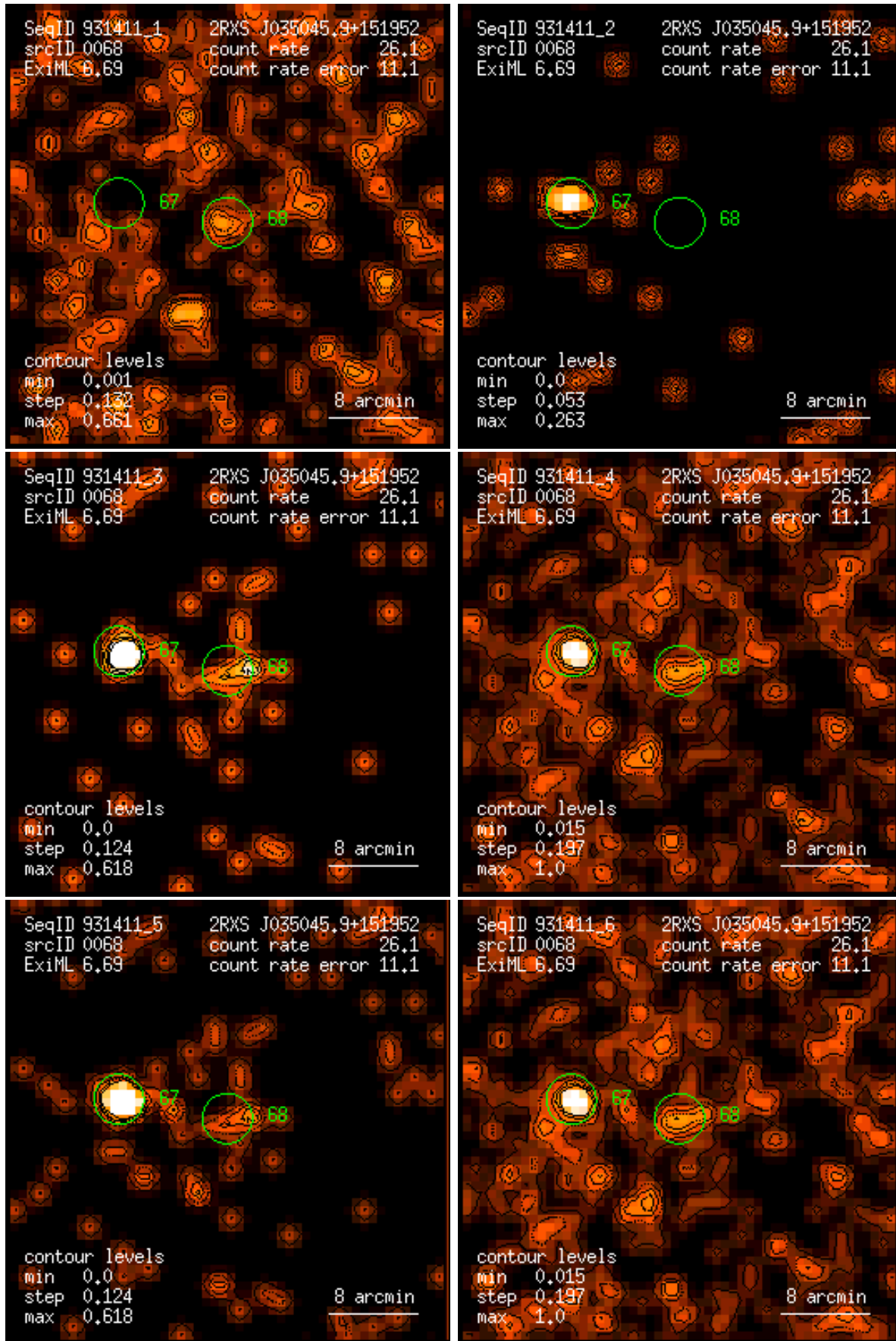
Figure 68: RASS 931411: detection 0068: band rate images, Gaussian filter: (1) PSPC channels 11 – 41, (2) 52 – 90, (3) 91 – 201, (4) 11 – 235, (5) 52 – 201, (6) 11 – 201. Broad band rates in counts/ks. Band rate contour levels in counts/ks/arcmin 2 .
