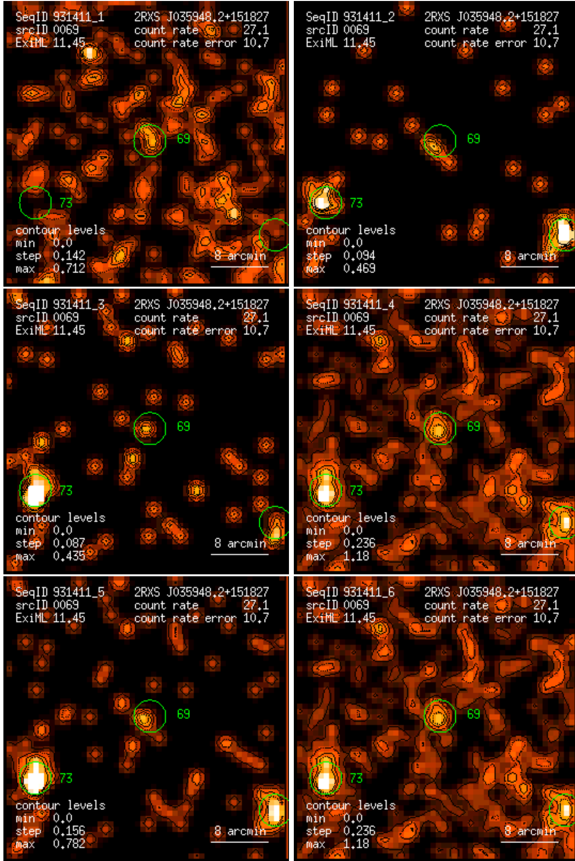
Figure 69: RASS 931411: detection 0069: band rate images, Gaussian filter: (1) PSPC channels 11 – 41, (2) 52 – 90, (3) 91 – 201, (4) 11 – 235, (5) 52 – 201, (6) 11 – 201. Broad band rates in counts/ks. Band rate contour levels in counts/ks/arcmin 2 .
